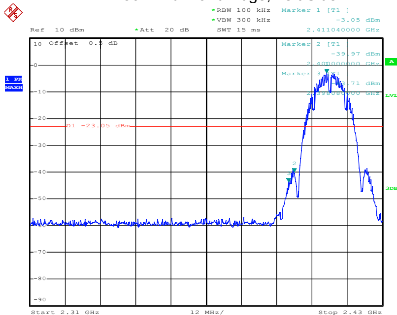
802.11b: Band Edge, Left Side
