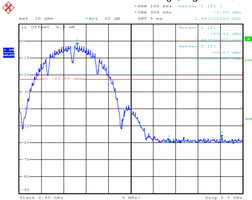
802.11b: Band Edge, Right Side
