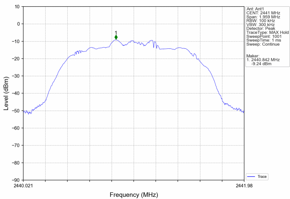
8-DPSK 3DH5 MCH 2441MHz_Ant1_NTNV
