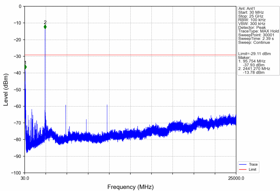
\pi/4 -DQPSK_2DH5_MCH_2441MHz_Ant1_NTNV
