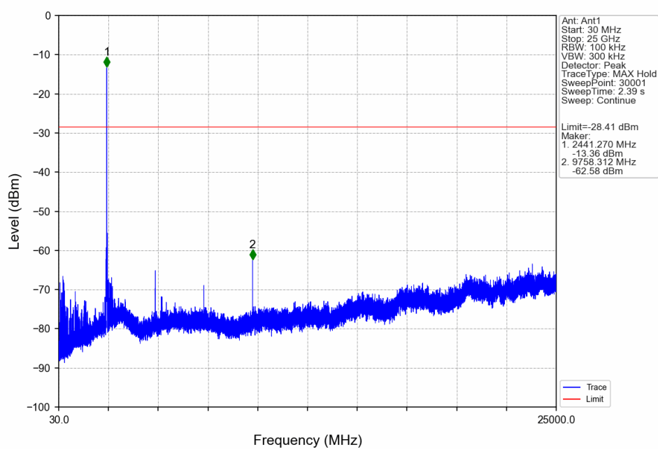
\pi/4 -DQPSK_2DH5_MCH_2441MHz_Ant1_NTNV
