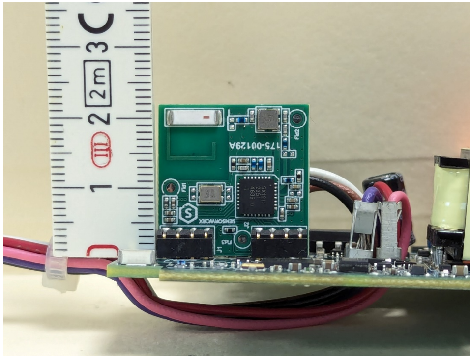
Top/Front of Daughter PCB mounted on Board
