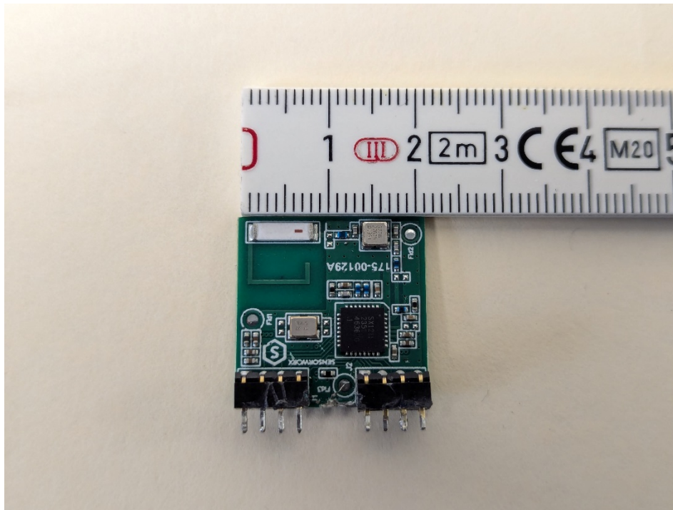
Bottom/Back of Daughter PCB
