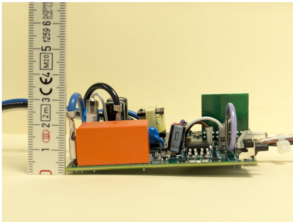
Side View of Main PCB and Daughter Card
