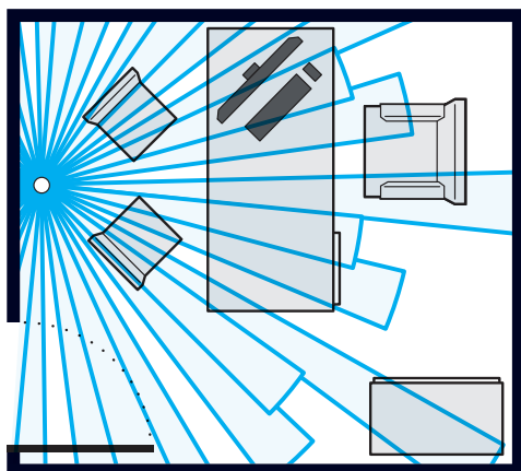
Diagram 1 - Recommended Sensor Placement in a Private Office
