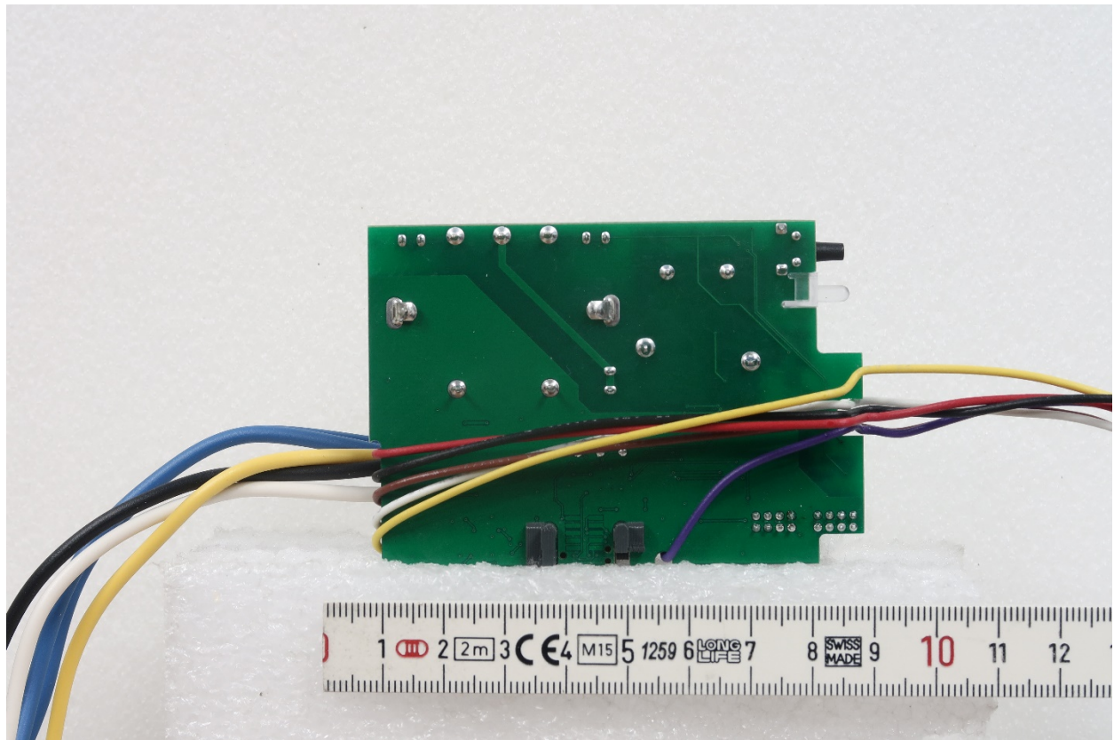
Mainboard Rear
