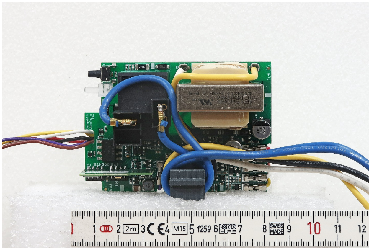
Mainboard Front
