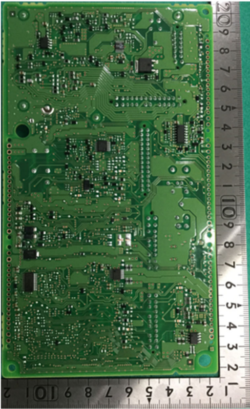
Solder side
