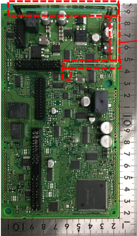
Component side
