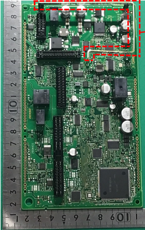
Component side
