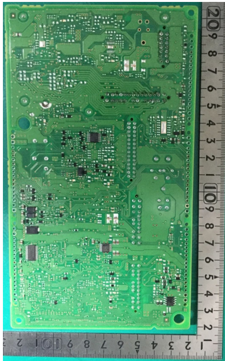
Solder side
