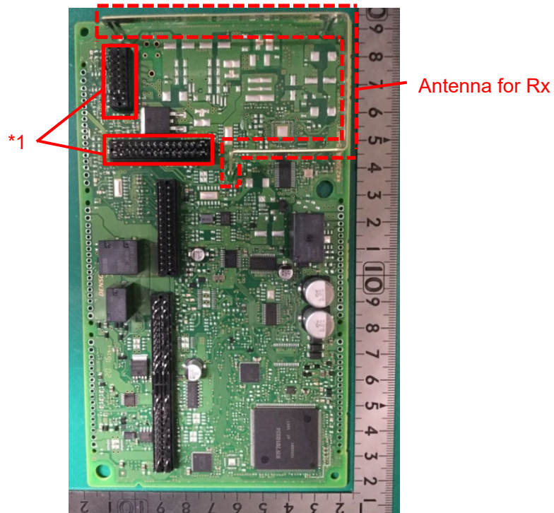
Component side
