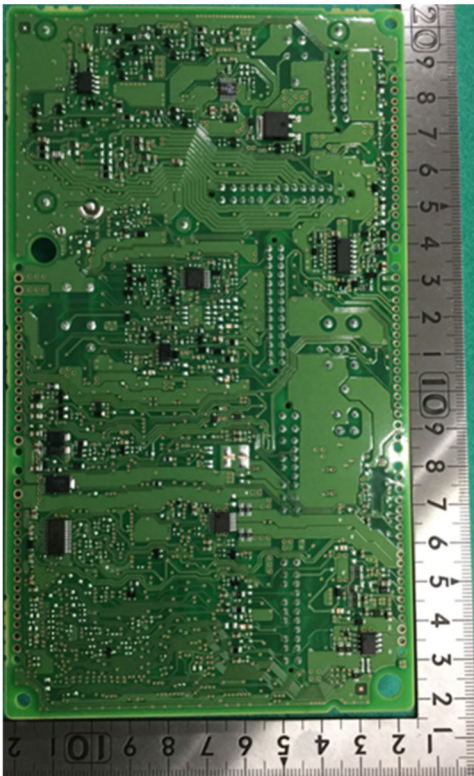
Solder side
