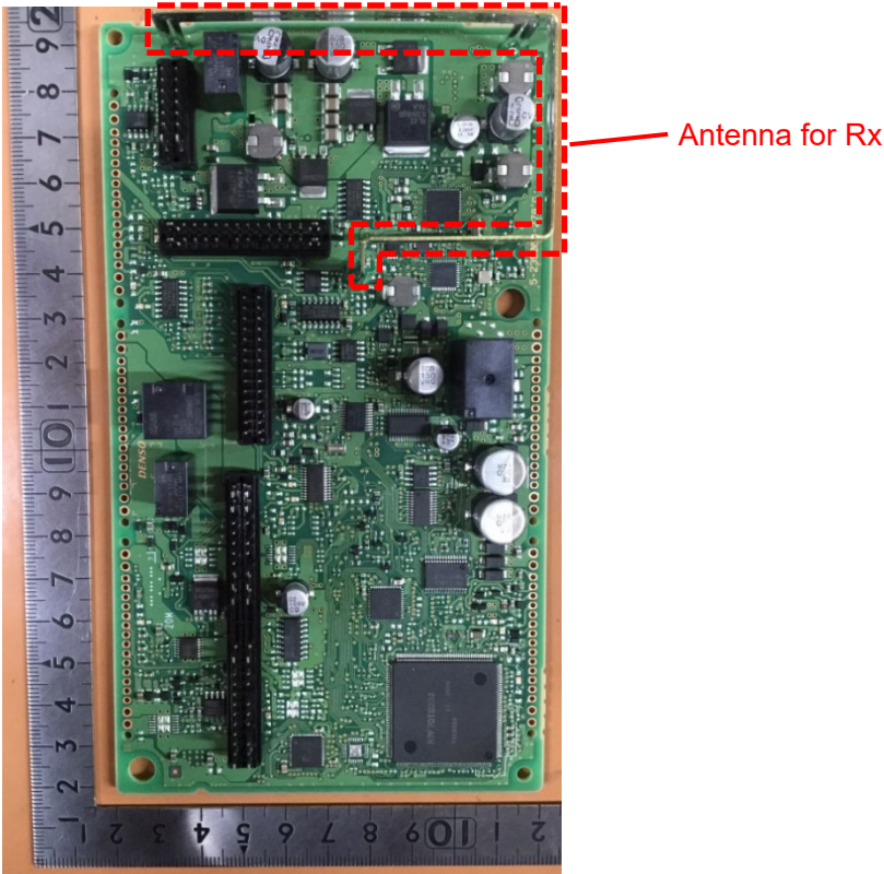
Component side
