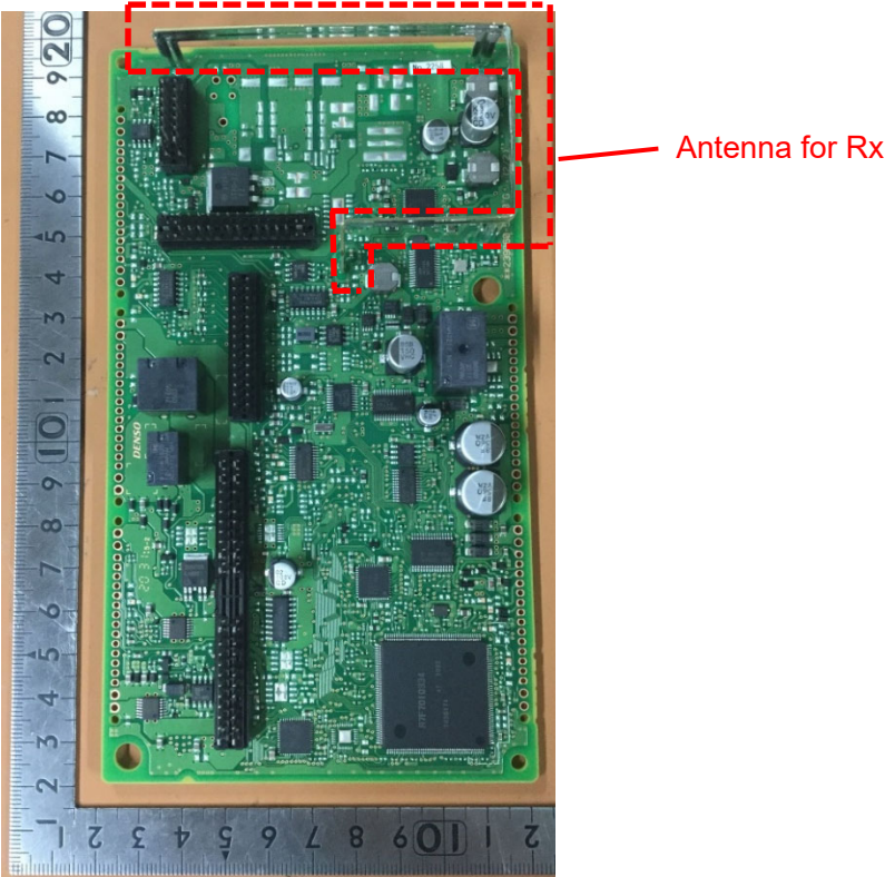
Component side
