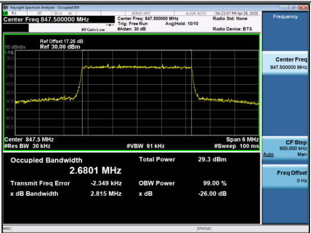
HCH_16QAM_15RB#0
