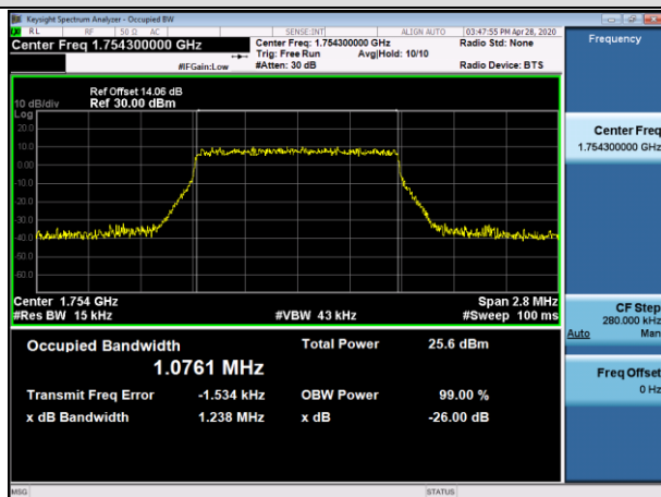
HCH_QPSK_6RB#0
