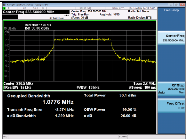
MCH_QPSK_6RB#0
