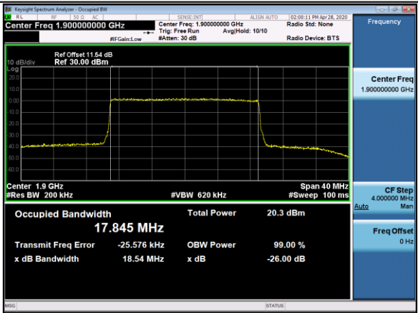
HCH_16QAM_100RB#0
