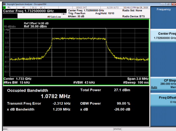
MCH_QPSK_6RB#0
