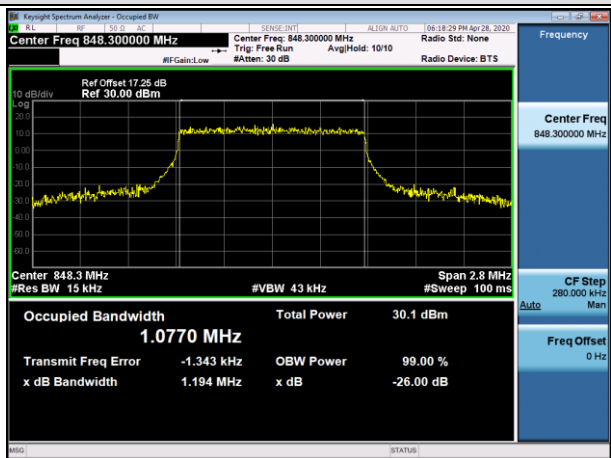
HCH_16QAM_6RB#0
