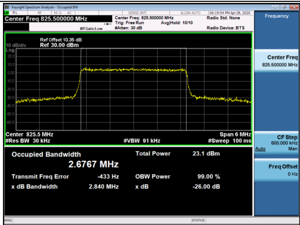
LCH_QPSK_15RB#0
