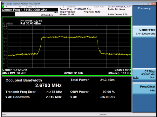
LCH_16QAM_15RB#0
