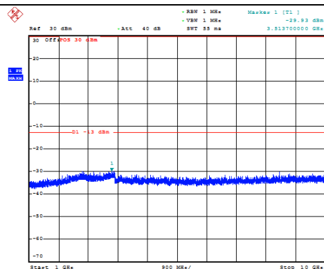
Channel 4175: 1GHz~10GHz
