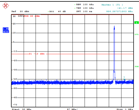
Channel 4133: 30MHz~1GHz
