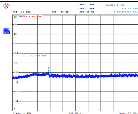
Channel 4133: 1GHz~10GHz
