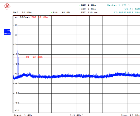
Channel 1450: 1GHz~20GHz
