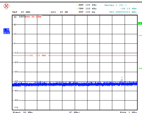
Channel 1450: 30MHz~1GHz
