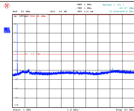
Channel 1312: 1GHz~20GHz
