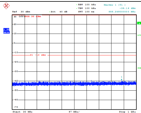
Channel 1512: 30MHz~1GHz
