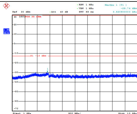
Channel 4232: 1GHz~10GHz
