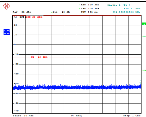
Channel 1312: 30MHz~1GHz
