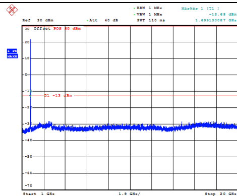
Channel 1512: 1GHz~20GHz
