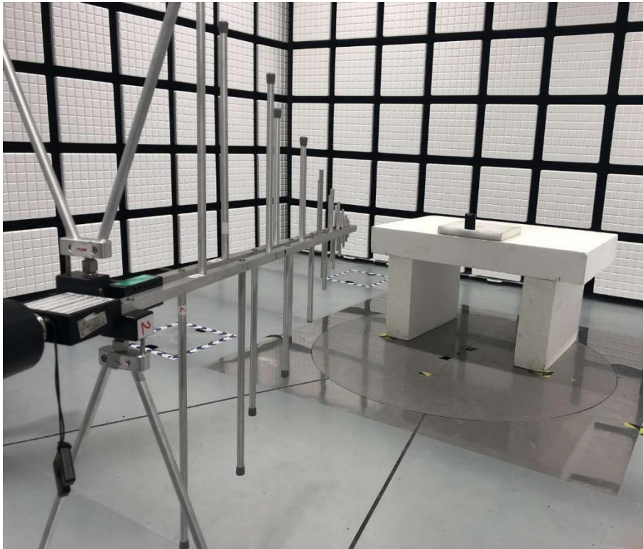
Picture2: Field Radiated Emissions (Above 30MHz)
