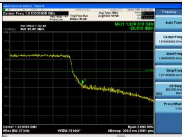
HCH_16QAM_6RB#0
