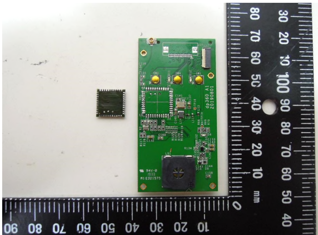
Internal View of EUT – 12
