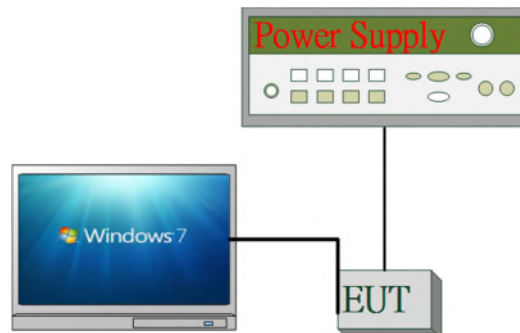
Fig. 2-3 Conducted (AC powerline) Emission Configuration
