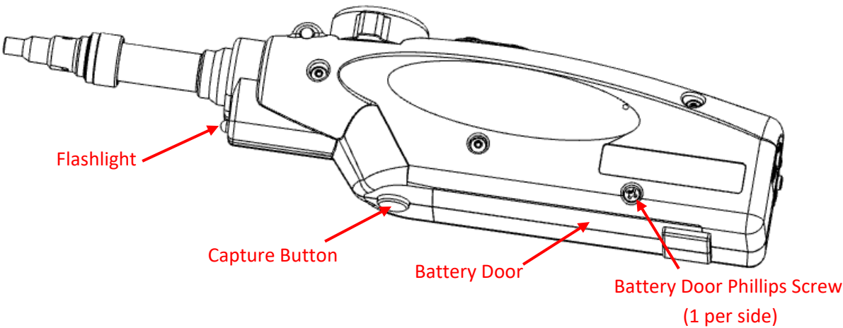
Figure 2 – Bottom View
