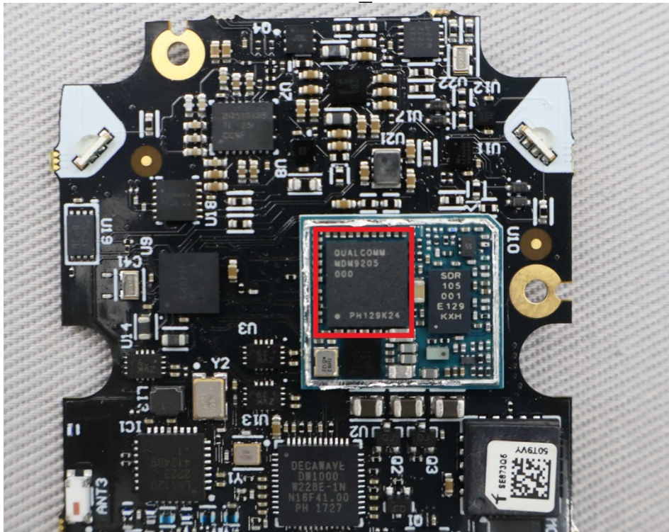
WWAN_IC
