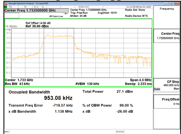
Band4_3MHz_16QAM_RB5_0_CH20385
