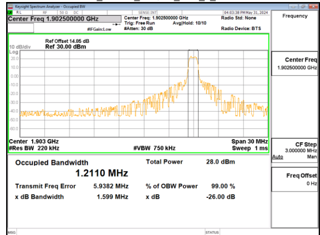
Band2_15MHz_16QAM_RB5_0_CH19125
