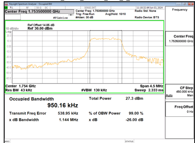
Band4_3MHz_16QAM_RB5_0_CH20385
