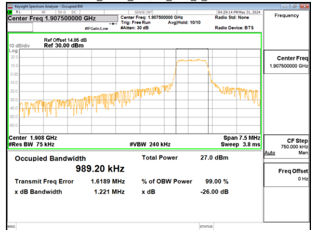
Band2_5MHz_16QAM_RB5_0_CH19175
