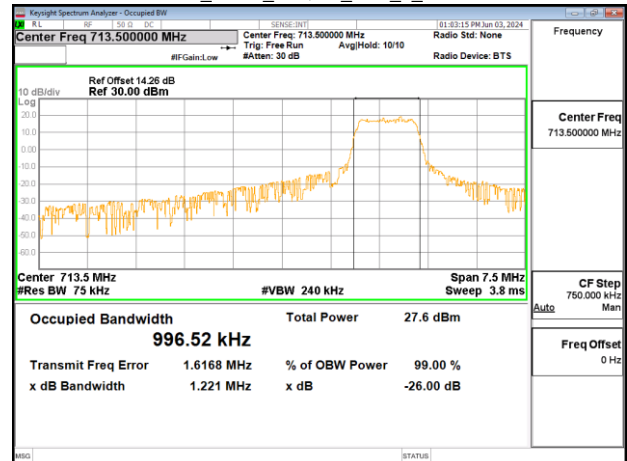
Band12_5MHz_16QAM_RB5_0_CH23155
