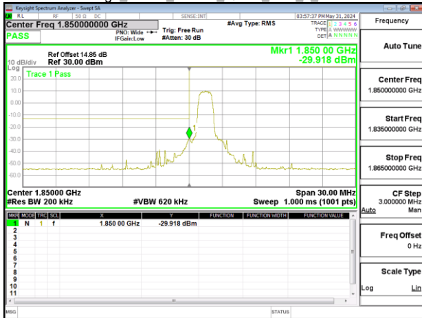
Band Edge_Band2_15MHz_QPSK_RB6_0_CH19125
