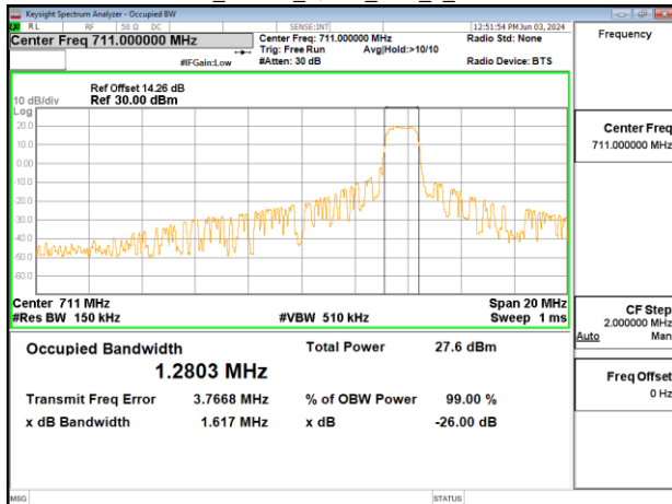
Band12_10MHz_QPSK_RB6_0_CH23130
