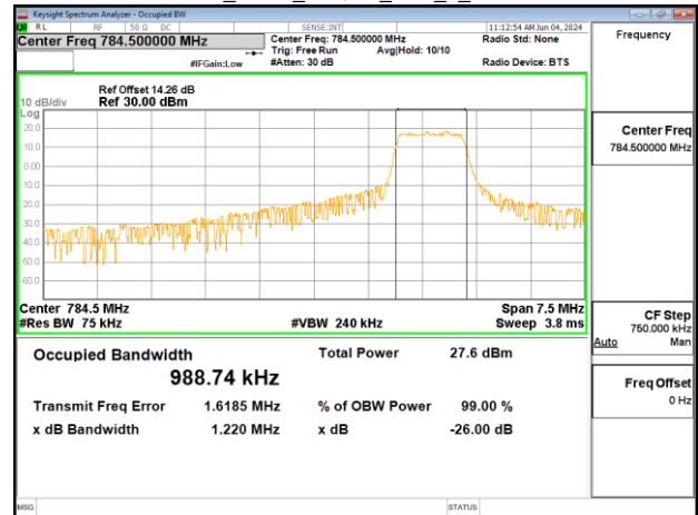
Band13_5MHz_16QAM_RB5_0_CH23255
