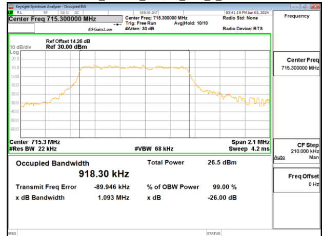
Band12_1.4MHz_16QAM_RB5_0_CH23173
