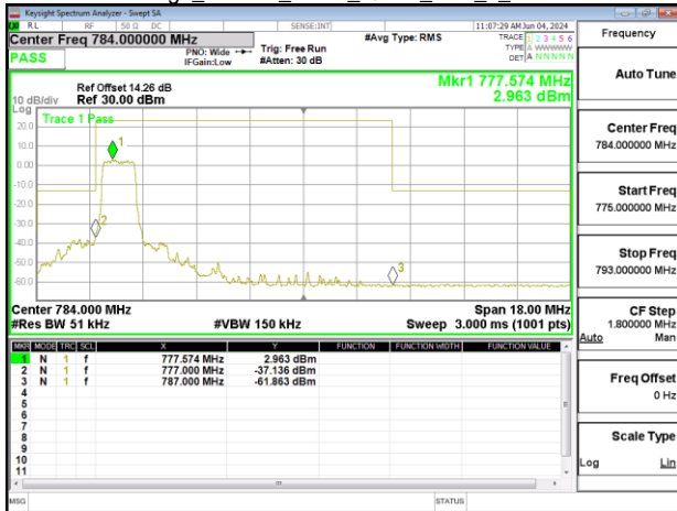
Band Edge_Band13_5MHz_QPSK_RB6_0_CH23255
