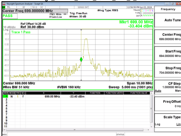
Band Edge_Band12_5MHz_QPSK_RB1_0_CH23035
