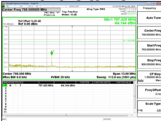
Band13_10MHz_QPSK_RB6_0_CH23230_index0
