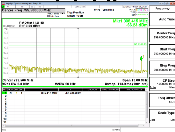
Band13_5MHz_QPSK_RB6_0_CH23205
