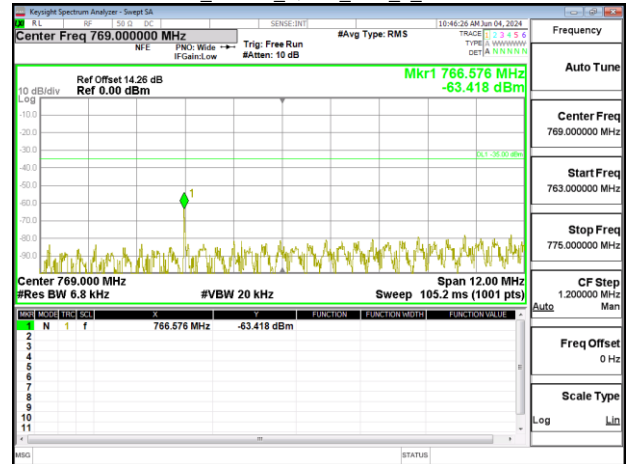
Band13_10MHz_QPSK_RB6_0_CH23230_index0
