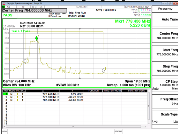
Band Edge_Band13_10MHz_QPSK_RB6_0_CH23230_index7
