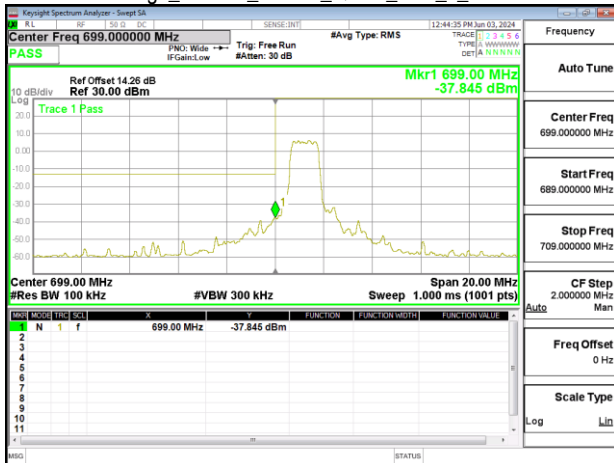
Band Edge_Band12_10MHz_QPSK_RB6_0_CH23060
