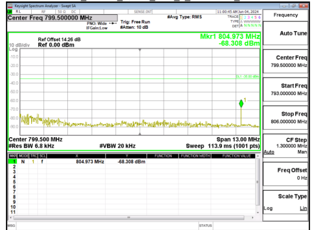
Band13_10MHz_QPSK_RB6_0_CH23230_index7
