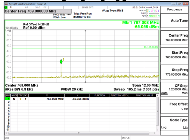
Band13_5MHz_QPSK_RB6_0_CH23255
