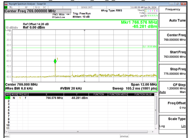
Band13_10MHz_QPSK_RB6_0_CH23230_index7
