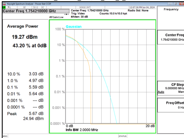
Band4_1.4MHz_16QAM_RB5_0_CH20393
