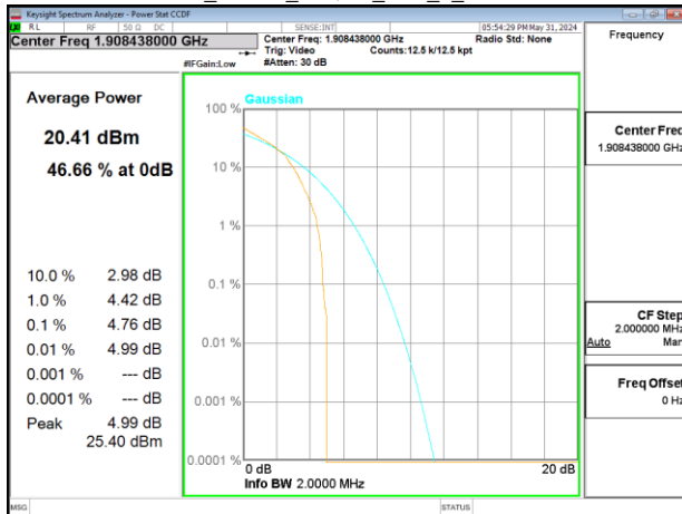
Band2_15MHz_16QAM_RB5_0_CH19125
