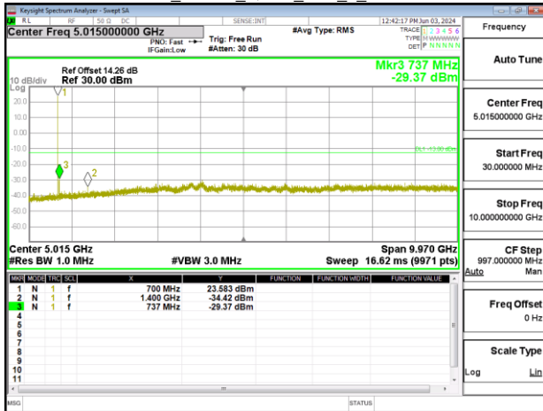
Band12_10MHz_QPSK_RB1_0_CH23095
