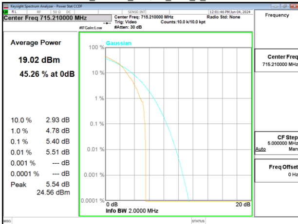
Band12_1.4MHz_16QAM_RB5_0_CH23173
