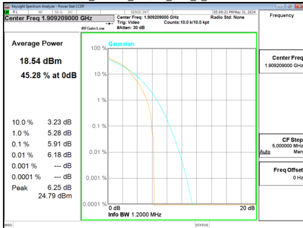
Band2_1.4MHz_16QAM_RB5_0_CH19193
