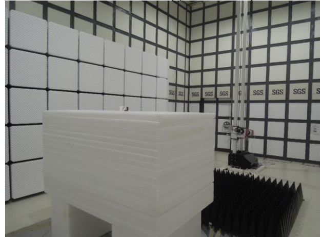
Cat-M1_Radiated_966(2)-E2 Plane.Setup
