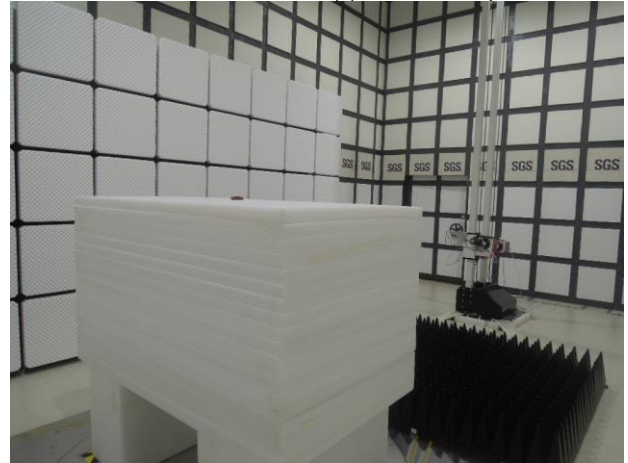
Cat-M1_Radiated_966(3)-E1 Plane.Setup
