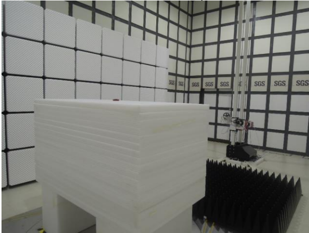
UWB_Radiated_Setup
