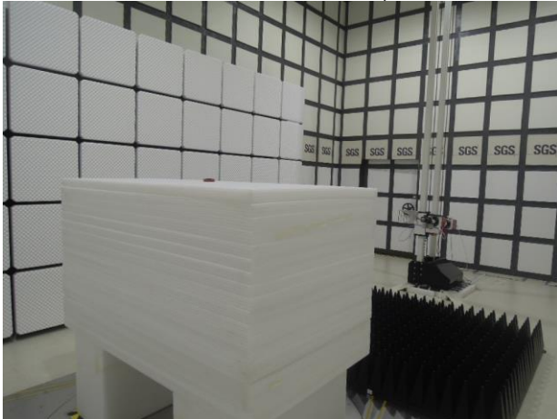
LoRaWAN_Radiated_Setup
