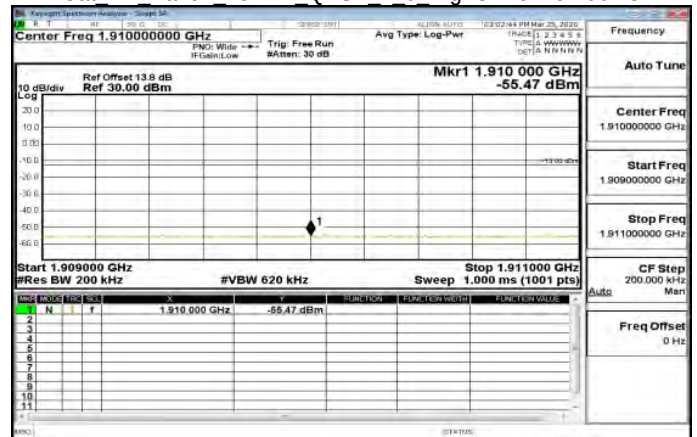
Cat M1 Band2 15MHz QPSK 1 0 HighCH19125-1902.5
