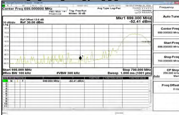
Cat M1 Band12 10MHz QPSK 6 0 LowCH23060-704
