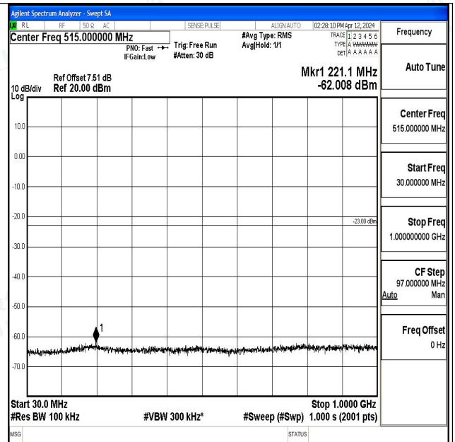
Band4_5MHz_16QAM_20175_1RB#0_30~1000_30~100
