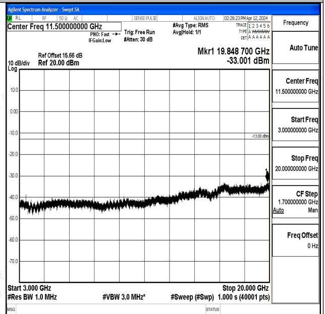
Band4_5MHz_16QAM_20175_1RB#0_3000~20000_300 0~20000
