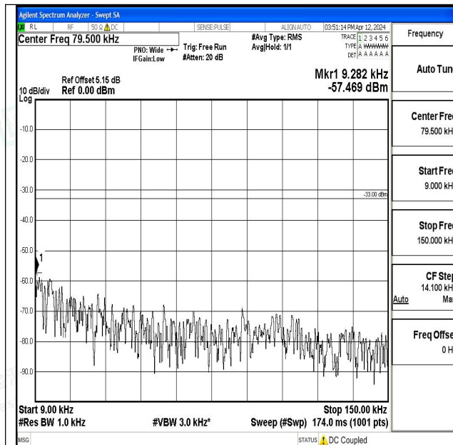
Band5_1.4MHz_QPSK_20407_1RB#0_0.009~0.15_0.00 9~0.15
