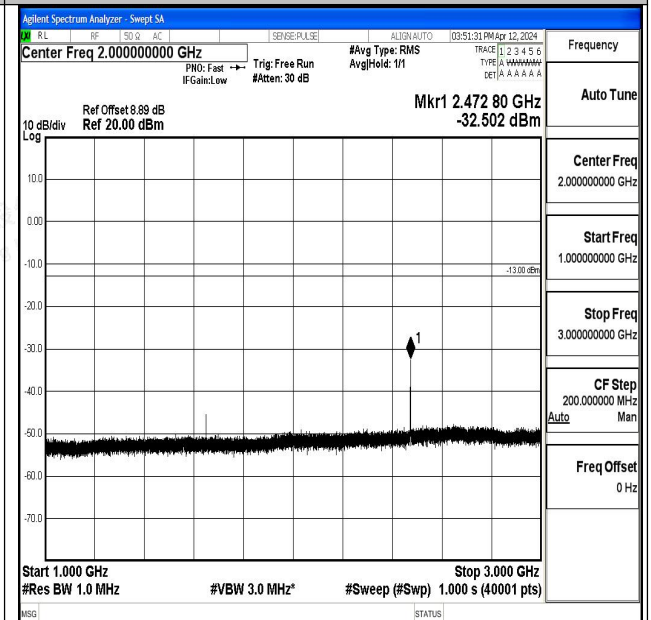
Band5_1.4MHz_QPSK_20407_1RB#0_1000~3000_1000 ~3000
