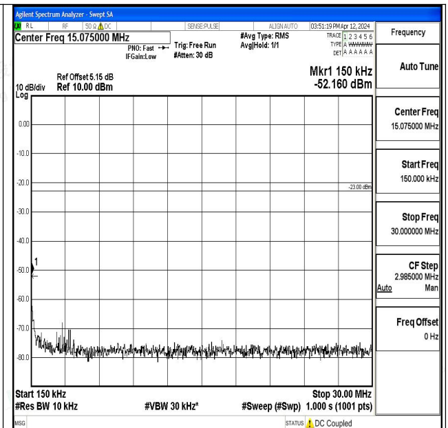
Band5_1.4MHz_QPSK_20407_1RB#0_0.15~30_0.15~30
