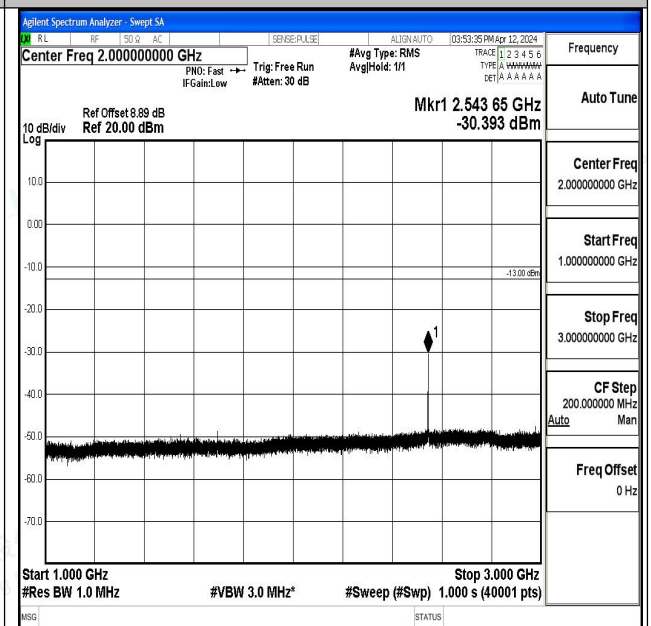
Band5_1.4MHz_QPSK_20643_1RB#0_1000~3000_1000 ~3000
