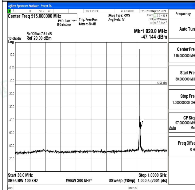
Band5_1.4MHz_QPSK_20407_1RB#0_30~1000_30~100 0
