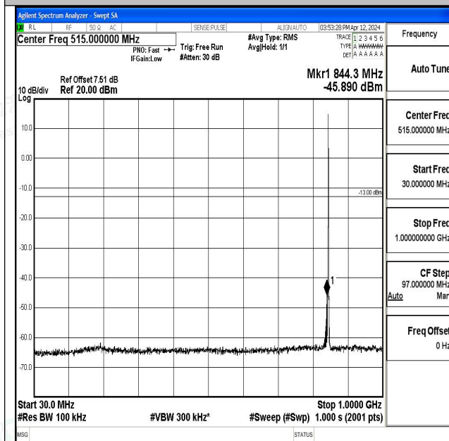
Band5_1.4MHz_QPSK_20643_1RB#0_30~1000_30~1000 0
