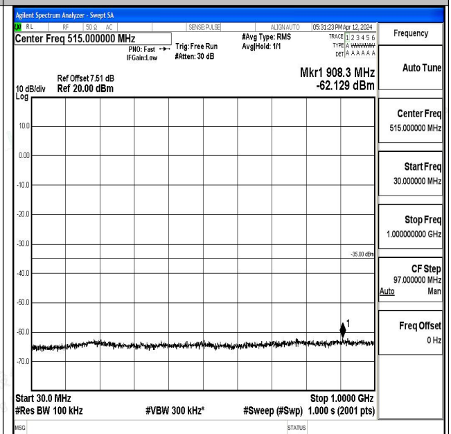
Band7_5MHz_16QAM_20775_1RB#0_30~1000_30~1000
