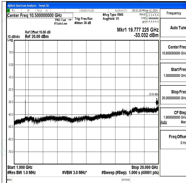
Band7_5MHz_16QAM_20775_1RB#0_1000~20000_100 0~20000
