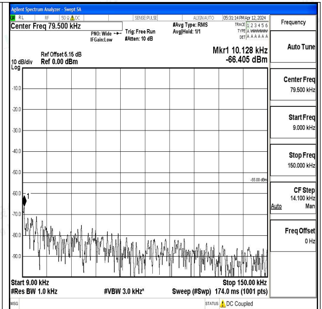
Band7_5MHz_16QAM_20775_1RB#0_0.009~0.15_0.009~0.15
