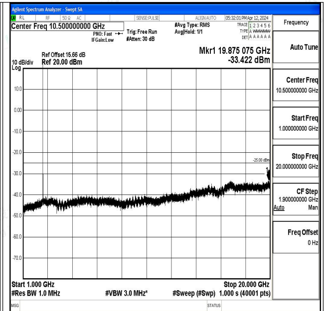
Band7_5MHz_QPSK_21100_1RB#0_1000~20000_1000~20000
