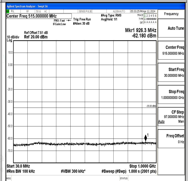
Band7_5MHz_16QAM_21425_1RB#0_30~1000_30~1000
