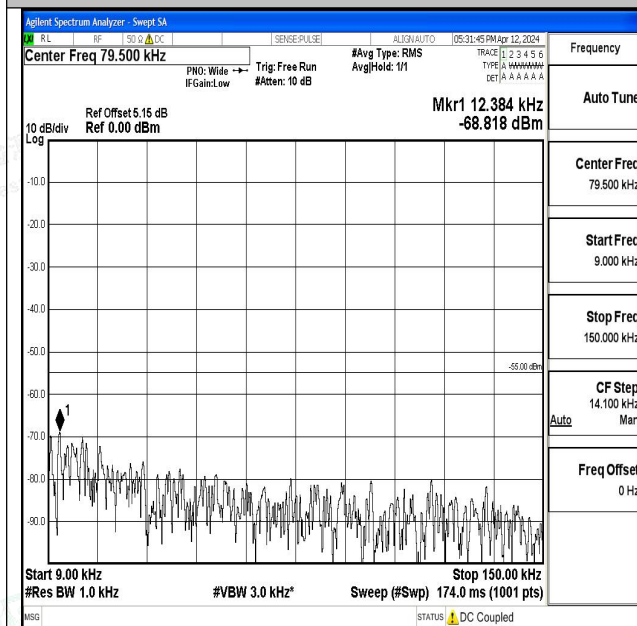
Band7_5MHz_QPSK_21100_1RB#0_0.009~0.15_0.009~ 0.15
