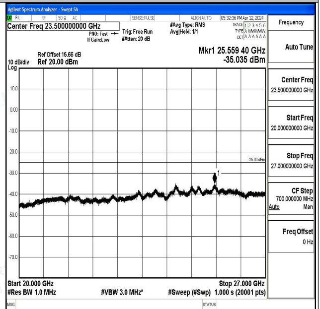
Band7_5MHz_16QAM_21100_1RB#0_20000~27000_20000~27000
