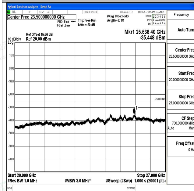
Band7_5MHz_QPSK_21100_1RB#0_20000~27000_20000~27000
