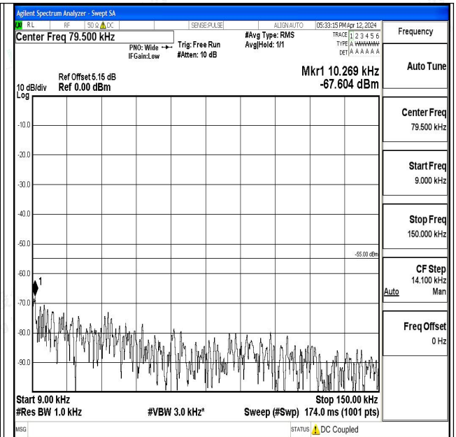
Band7_5MHz_16QAM_21425_1RB#0_0.009~0.15_0.009~0.15
