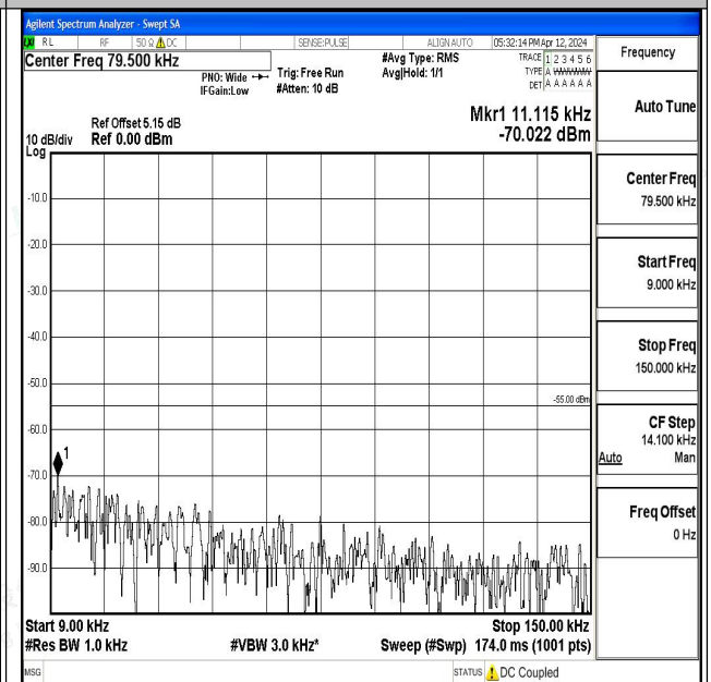
Band7_5MHz_16QAM_21100_1RB#0_0.009~0.15_0.009~0.15
