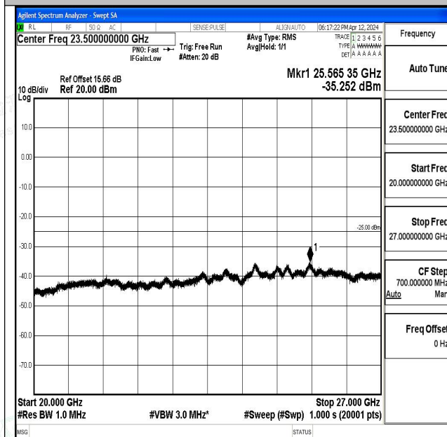
Band7_15MHz_QPSK_21100_1RB#0_20000~27000_20
