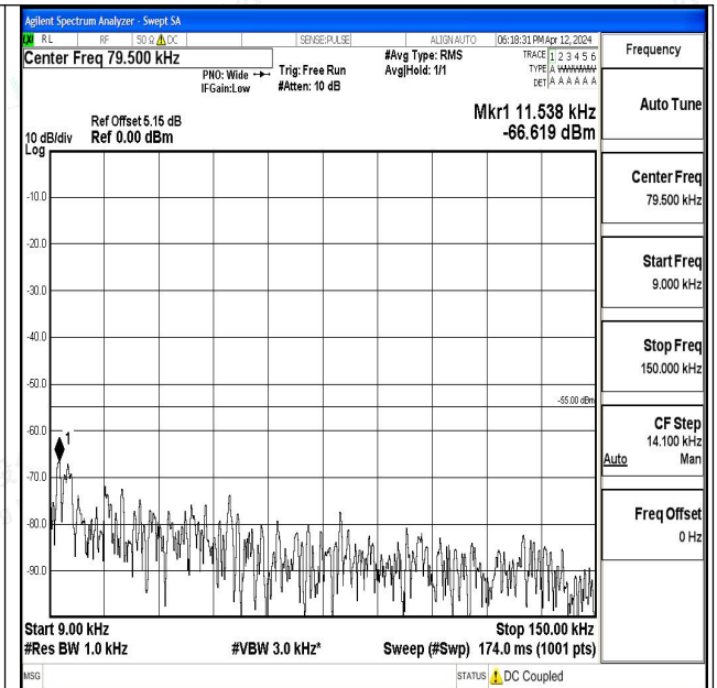
Band7_15MHz_16QAM_21375_1RB#0_0.009~0.15_0.0 09~0.15
