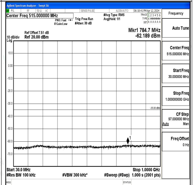
Band7_15MHz_16QAM_21375_1RB#0_30~1000_30~10 00
