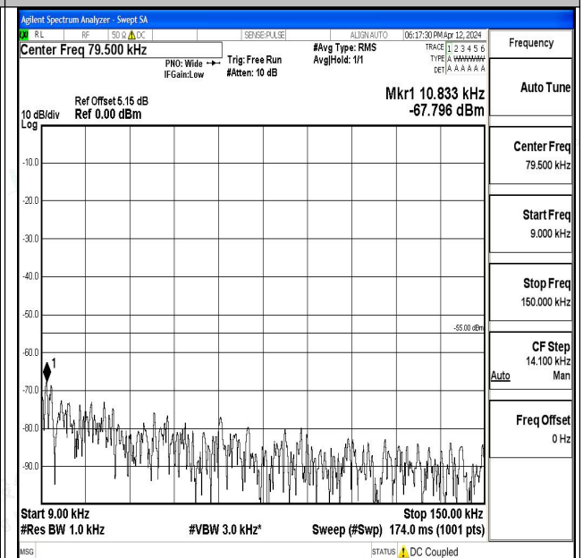
Band7_15MHz_16QAM_21100_1RB#0_0.009~0.15_0.00
