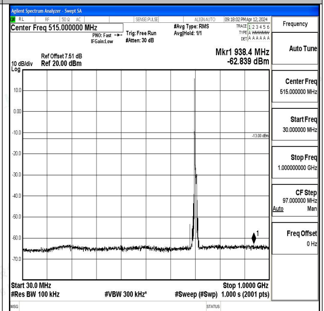
Band17_10MHz_16QAM_23790_1RB#0_30~1000_30~1 000
