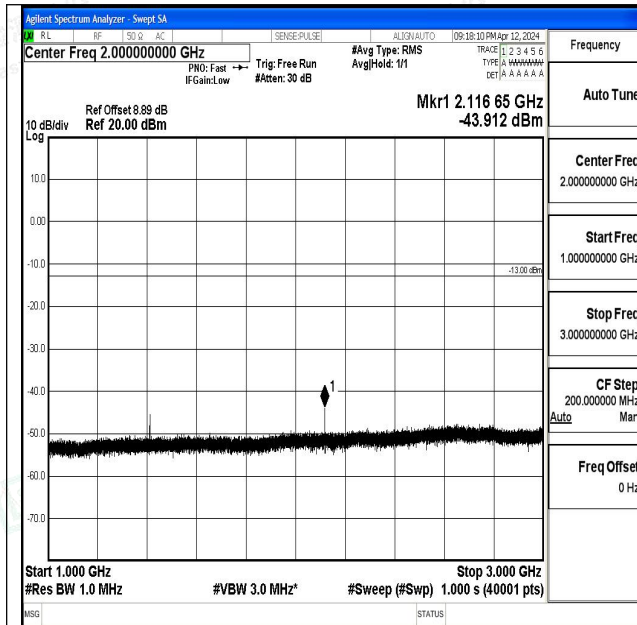
Band17_10MHz_16QAM_23790_1RB#0_1000~3000_10 00~3000
