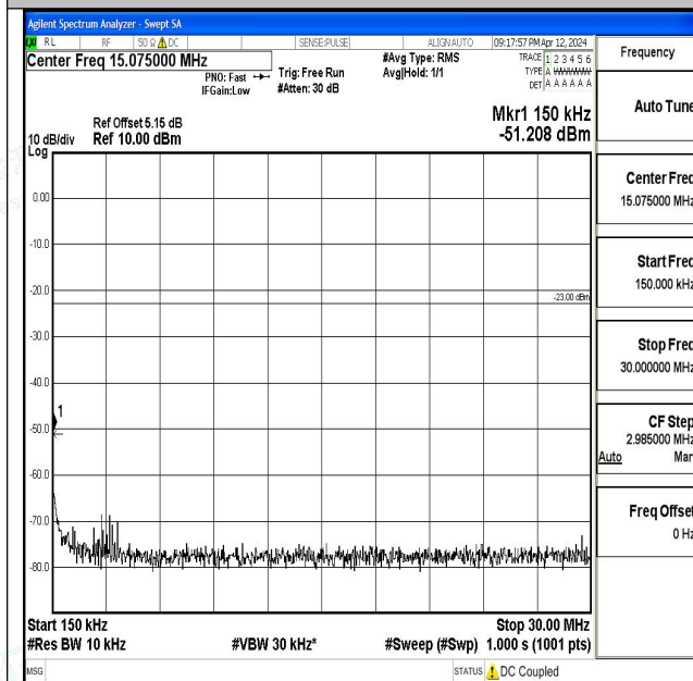
Band17_10MHz_16QAM_23790_1RB#0_0.15~30_0.15~ 30
