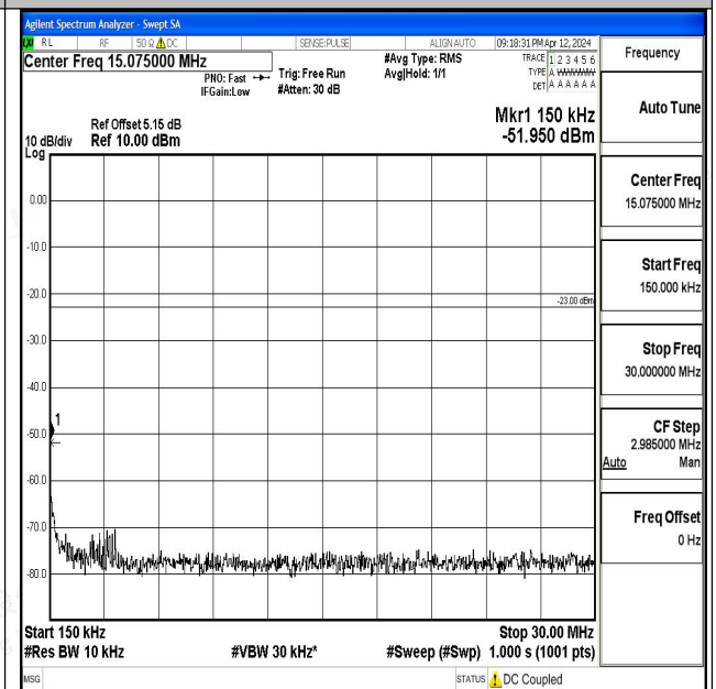
Band17_10MHz_QPSK_23800_1RB#0_0.15~30_0.15~3 0
