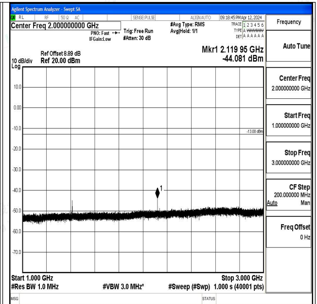
Band17_10MHz_QPSK_23800_1RB#0_1000~3000_100 0~3000
