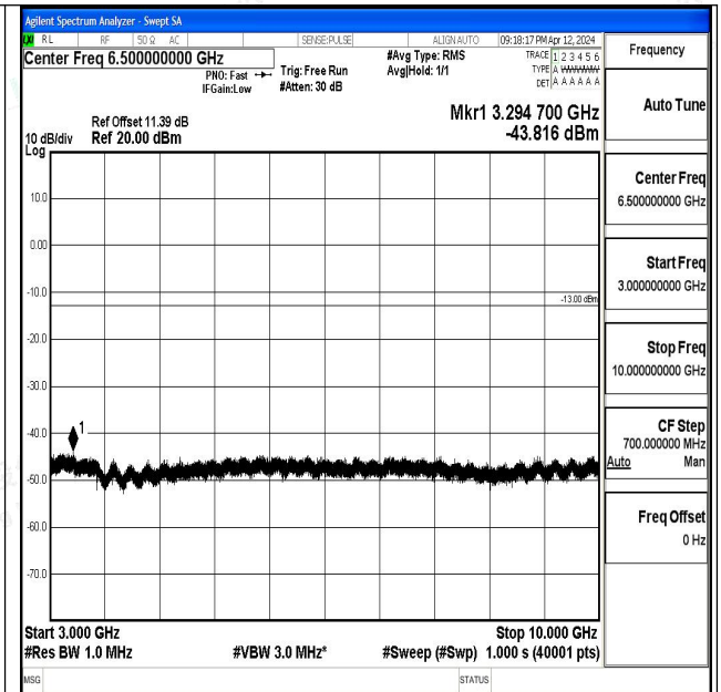
Band17_10MHz_16QAM_23790_1RB#0_3000~10000_3 000~10000
