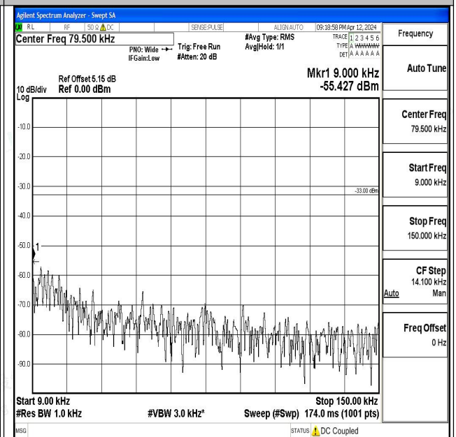
Band17_10MHz_16QAM_23800_1RB#0_0.009~0.15_0. 009~0.15
