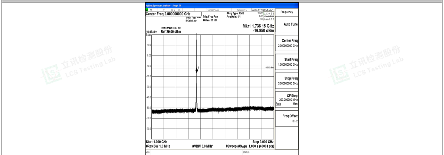
Band4_1.4MHz_16QAM_20175_1RB#0_1000~3000_1000~3000
