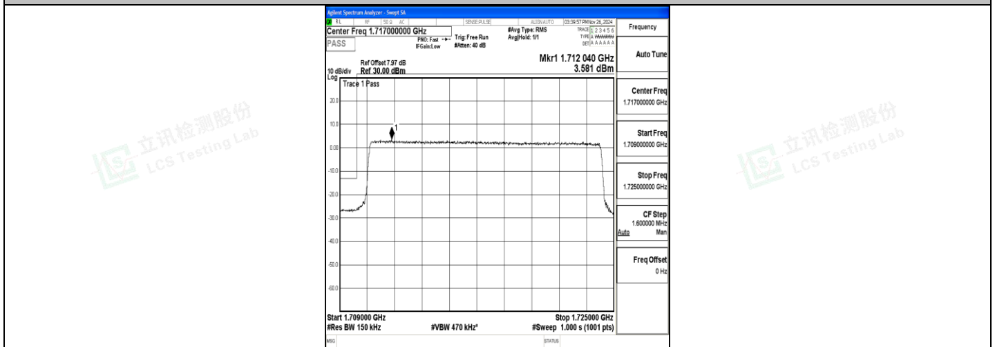
Band4_15MHz_16QAM_20025_75RB#0
