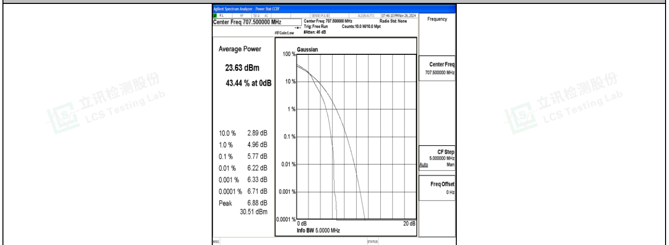
Band12-5MHz-16QAM-23095-1RB#0-PASS
