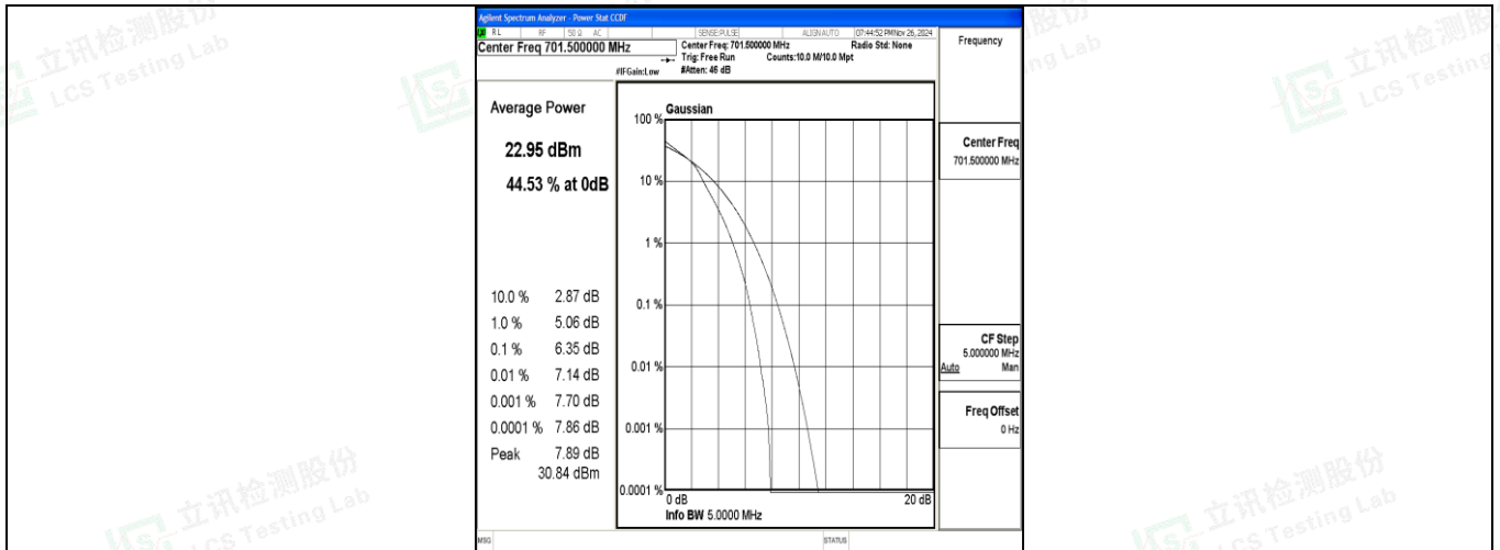
Band12-5MHz-16QAM-23035-25RB#0-PASS
