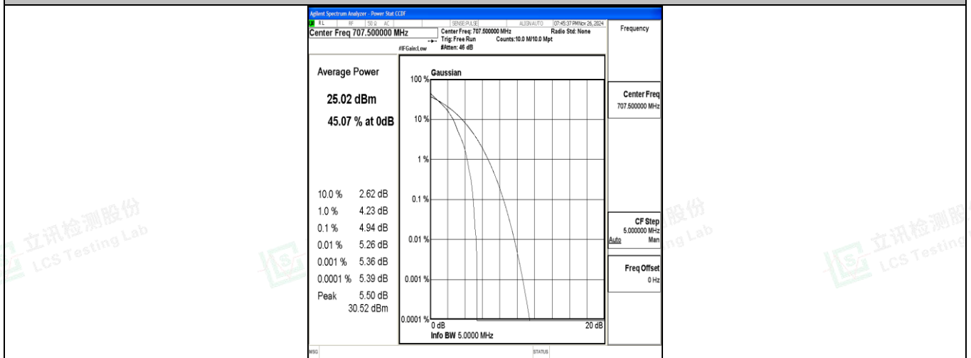
Band12-5MHz-QPSK-23095-1RB#0-PASS
