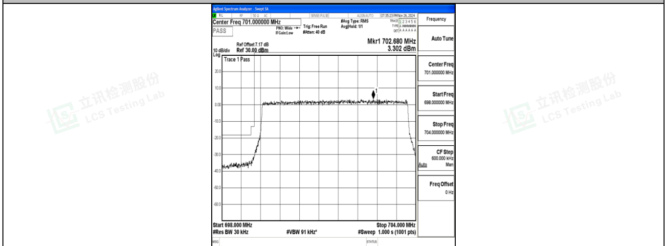
Band12_5MHz_16QAM_23035_25RB#0
