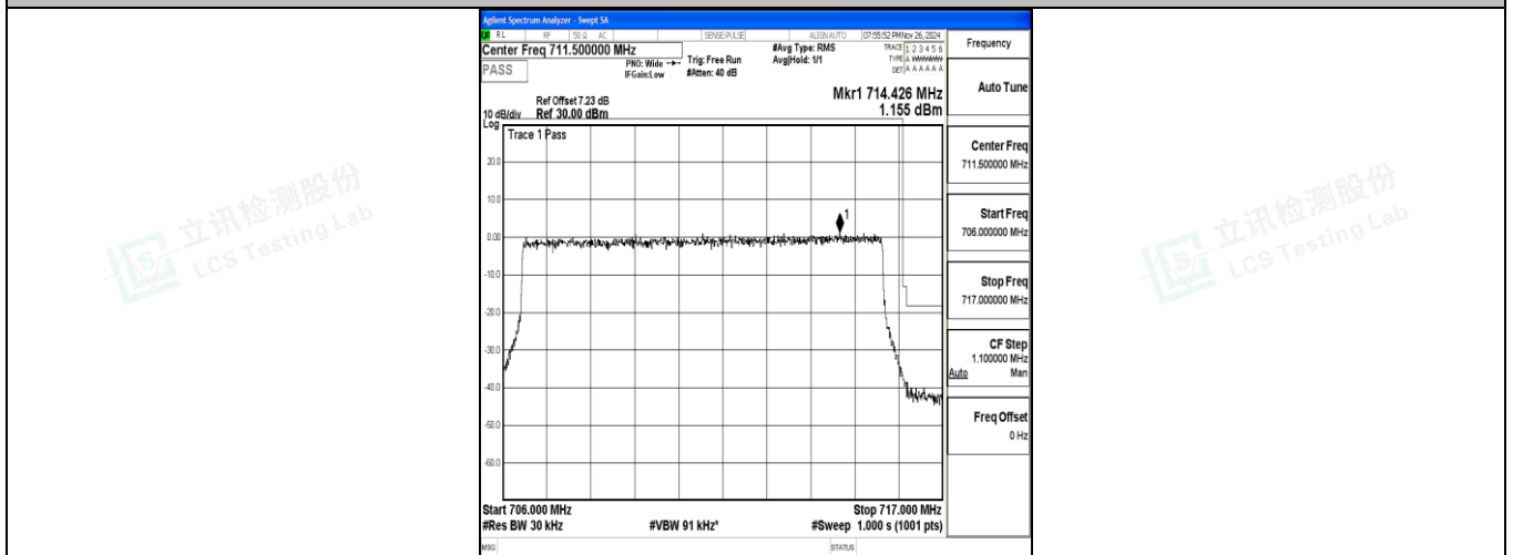
Band12_10MHz_16QAM_23130_50RB#0
