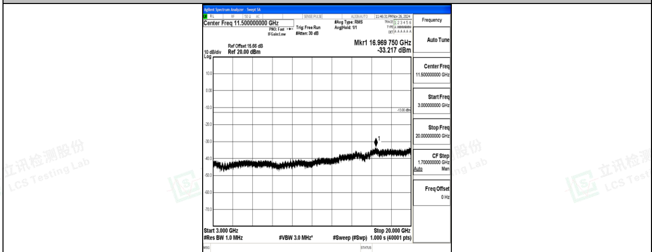
Band66_1.4MHz_16QAM_132665_1RB#0_3000~20000_3000~20000
