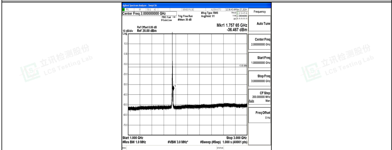
Band66_5MHz_16QAM_132322_1RB#0_1000~3000_1000~3000
