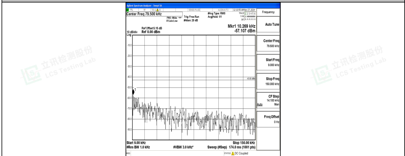
Band66_3MHz_QPSK_131987_1RB#0_0.009~0.15_0.009~0.15
