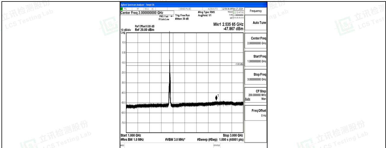
Band66_10MHz_QPSK_132322_1RB#0_1000~3000_1000~3000
