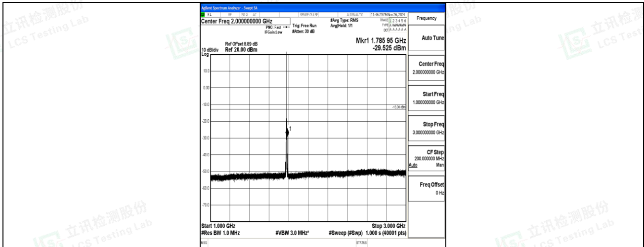
Band66_1.4MHz_16QAM_132665_1RB#0_1000~3000_1000~3000
