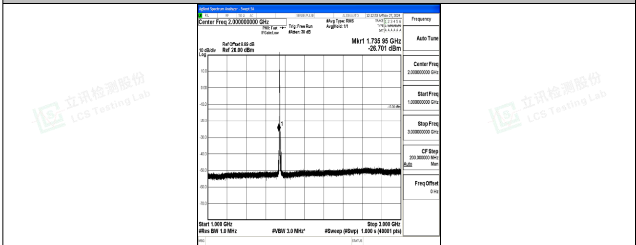
Band66_3MHz_16QAM_132322_1RB#0_1000~3000_1000~3000
