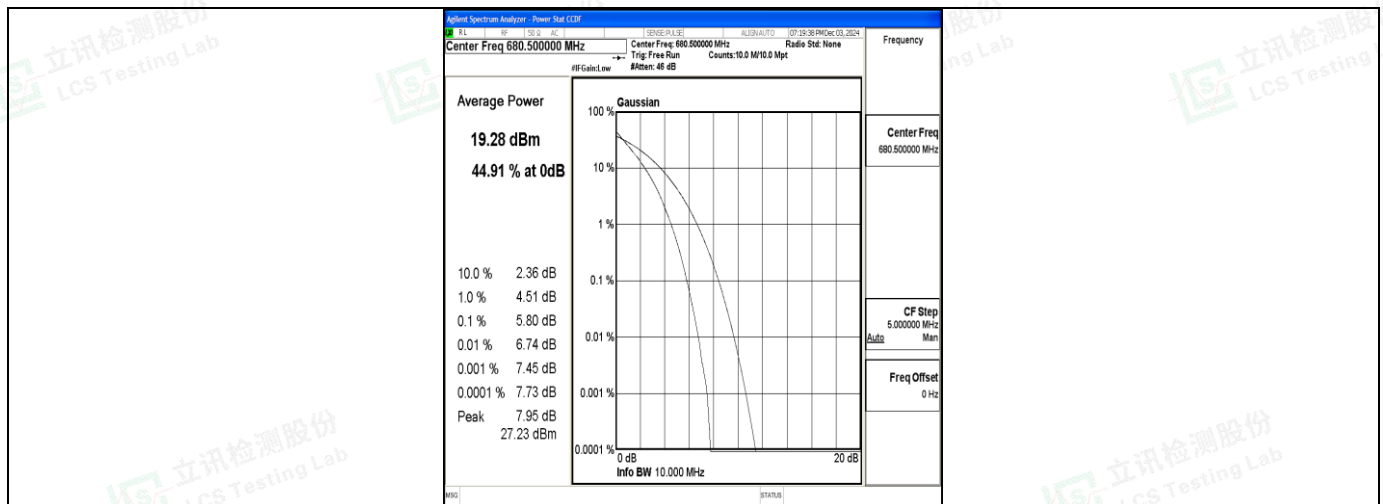
Band71-10MHz-QPSK-133297-50RB#0-PASS
