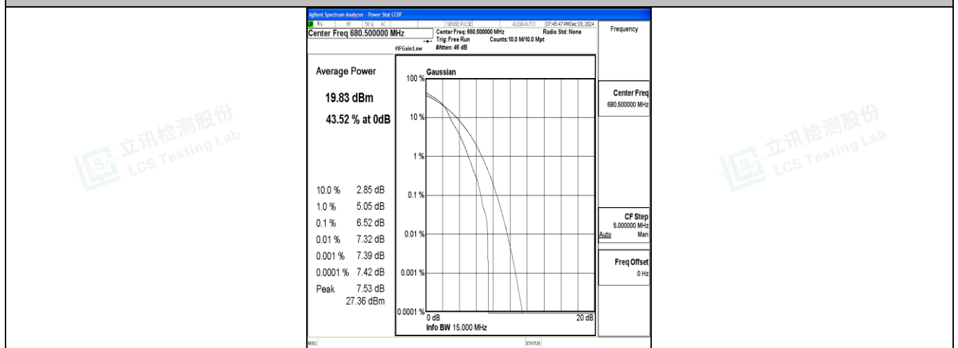
Band71-15MHz-16QAM-133297-1RB#0-PASS
