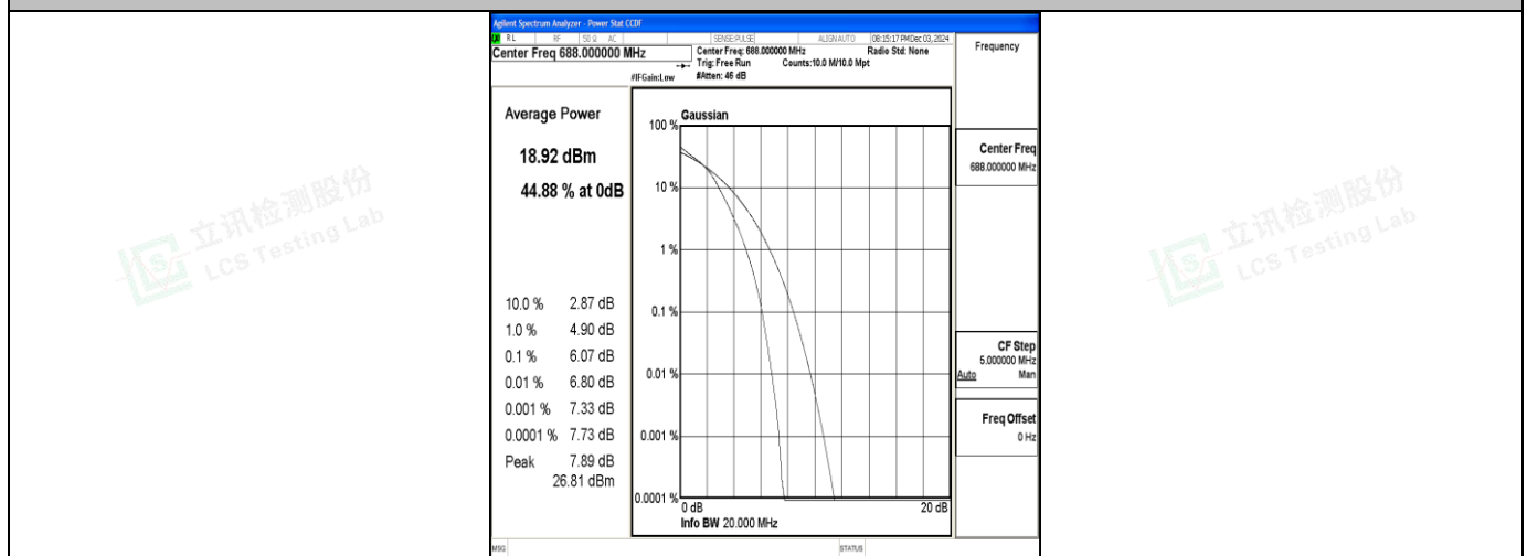
Band71-20MHz-16QAM-133372-100RB#0-PASS
