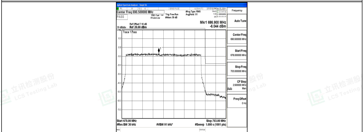
Band71_20MHz_QPSK_133372_100RB#0
