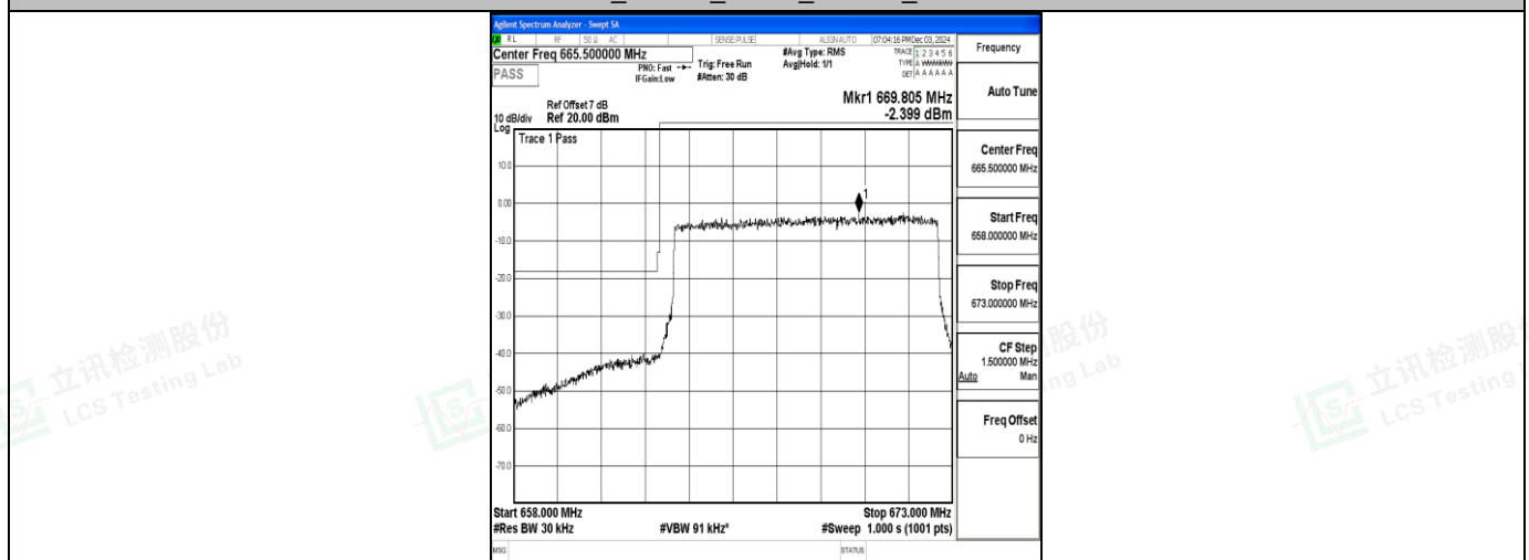
Band71_10MHz_16QAM_133172_50RB#0
