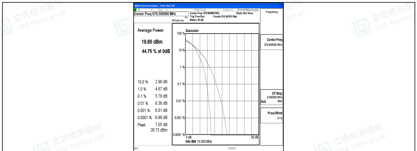
Band71-15MHz-16QAM-133197-75RB#0-PASS
