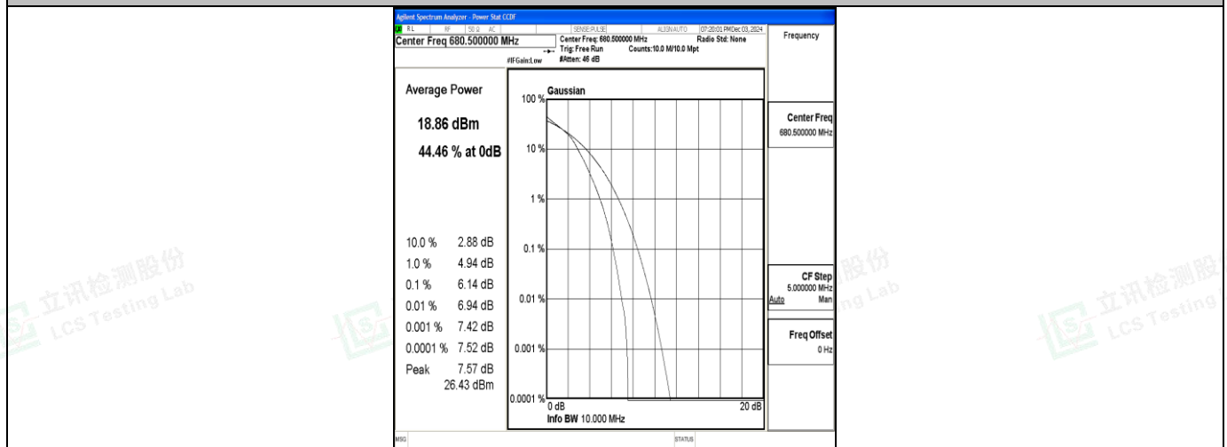
Band71-10MHz-16QAM-133297-50RB#0-PASS
