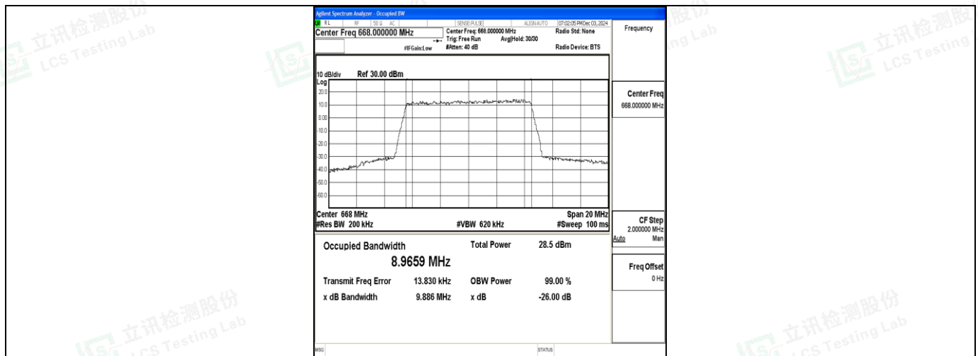
Band71-10MHz-QPSK-133172-50RB#0-PASS
