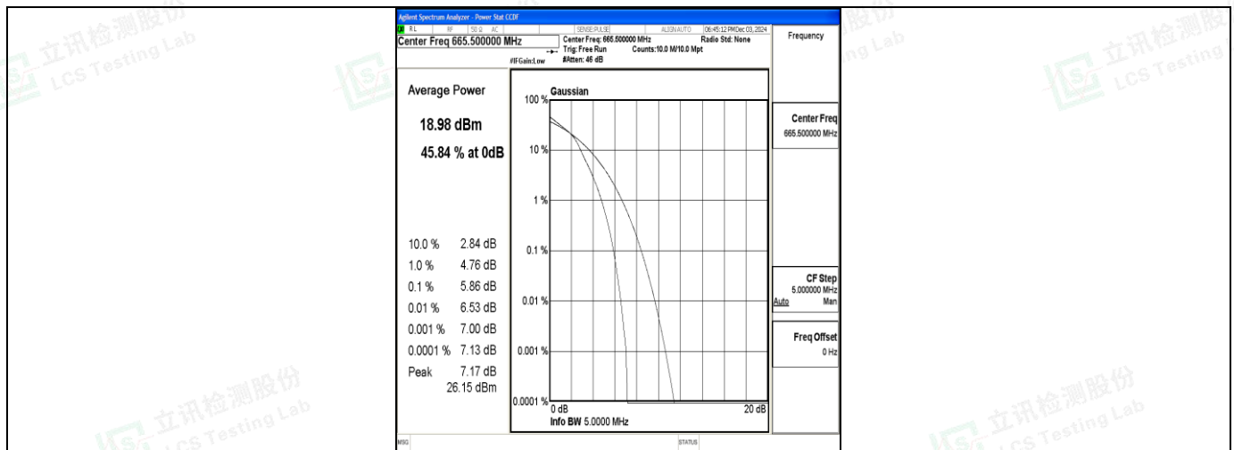
Band71-5MHz-16QAM-133147-25RB#0-PASS
