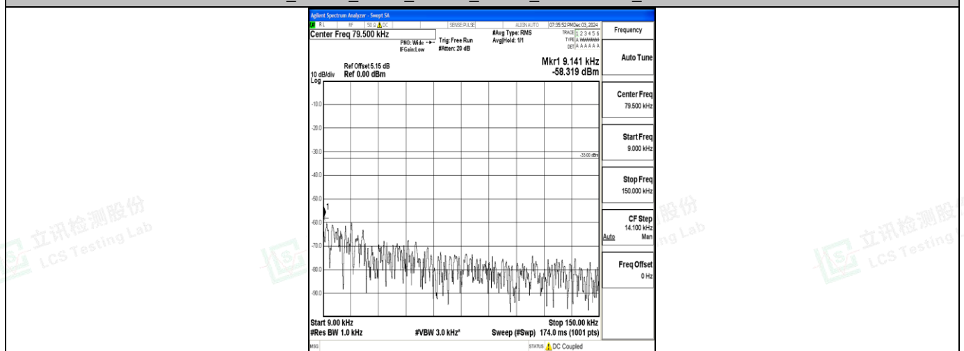
Band71_15MHz_16QAM_133297_1RB#0_0.009~0.15_0.009~0.15
