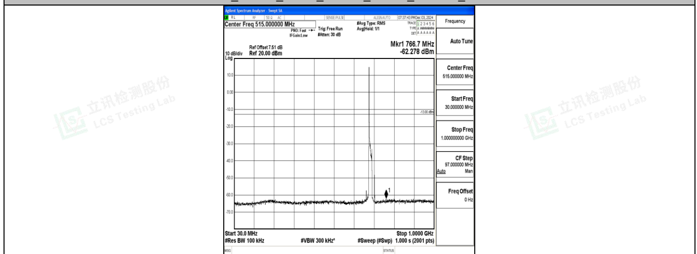
Band71_15MHz_QPSK_133397_1RB#0_30~1000_30~1000
