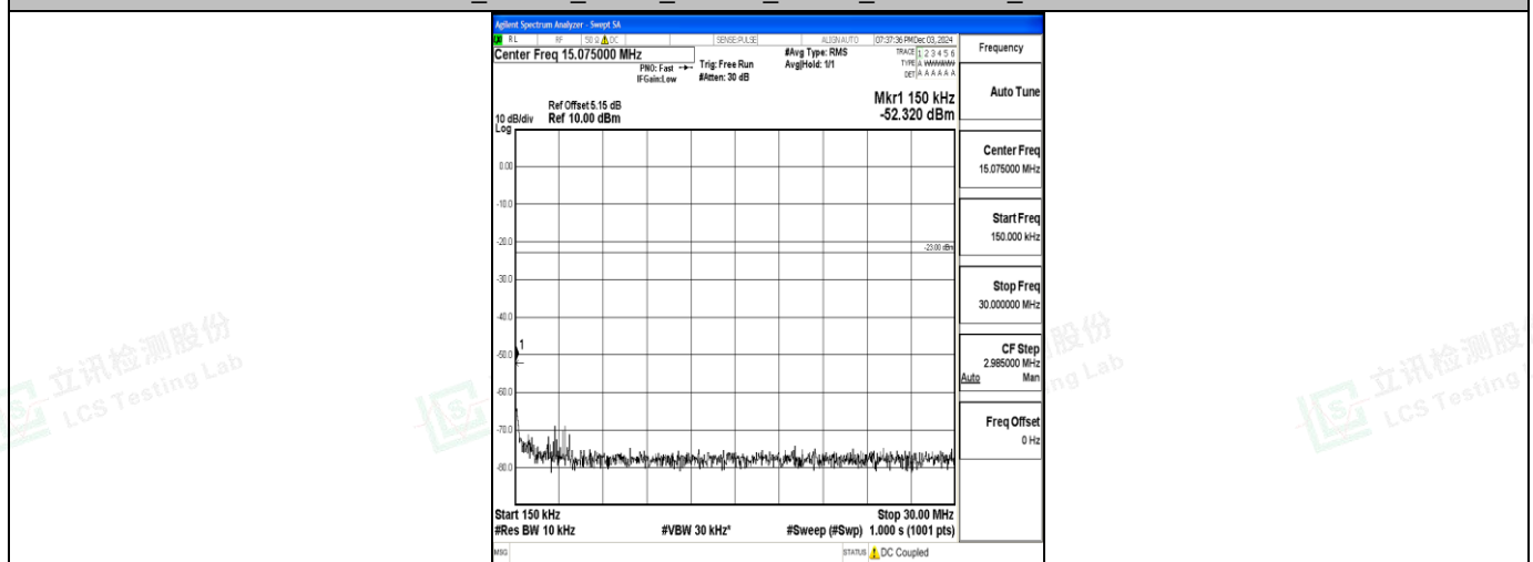
Band71_15MHz_QPSK_133397_1RB#0_0.15~30_0.15~30
