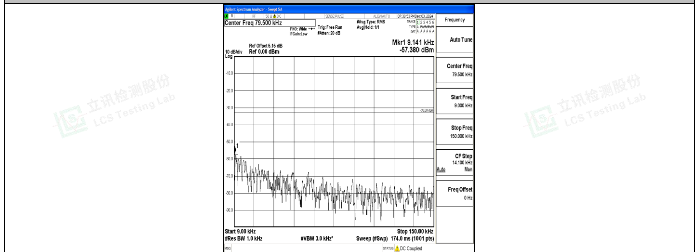
Band71_15MHz_16QAM_133397_1RB#0_0.009~0.15_0.009~0.15
