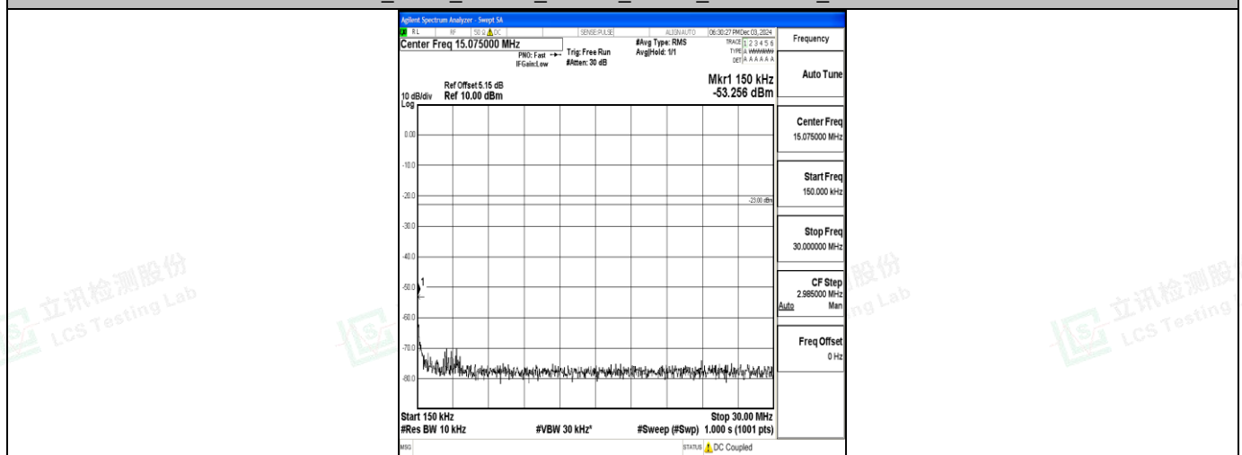
Band71_5MHz_16QAM_133147_1RB#0_0.15~30_0.15~30
