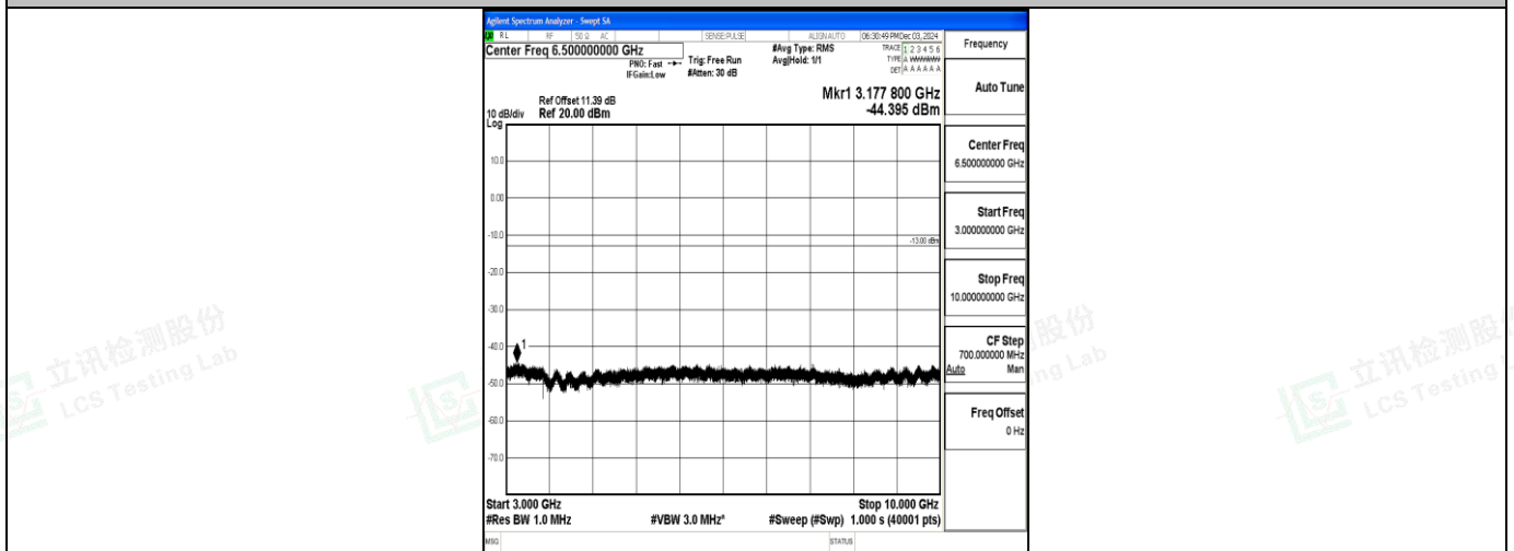
Band71_5MHz_16QAM_133147_1RB#0_3000~10000_3000~10000
