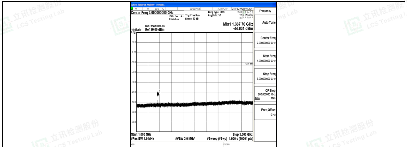
Band71_15MHz_QPSK_133397_1RB#0_1000~3000_1000~3000
