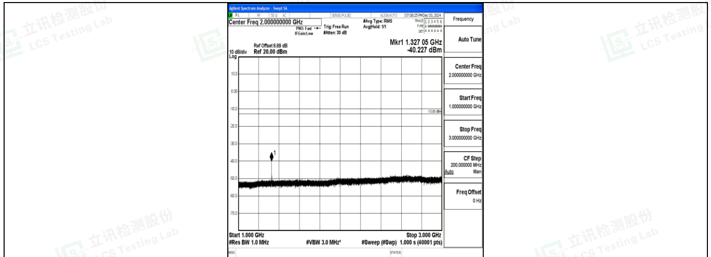
Band71_10MHz_16QAM_133172_1RB#0_1000~3000_1000~3000
