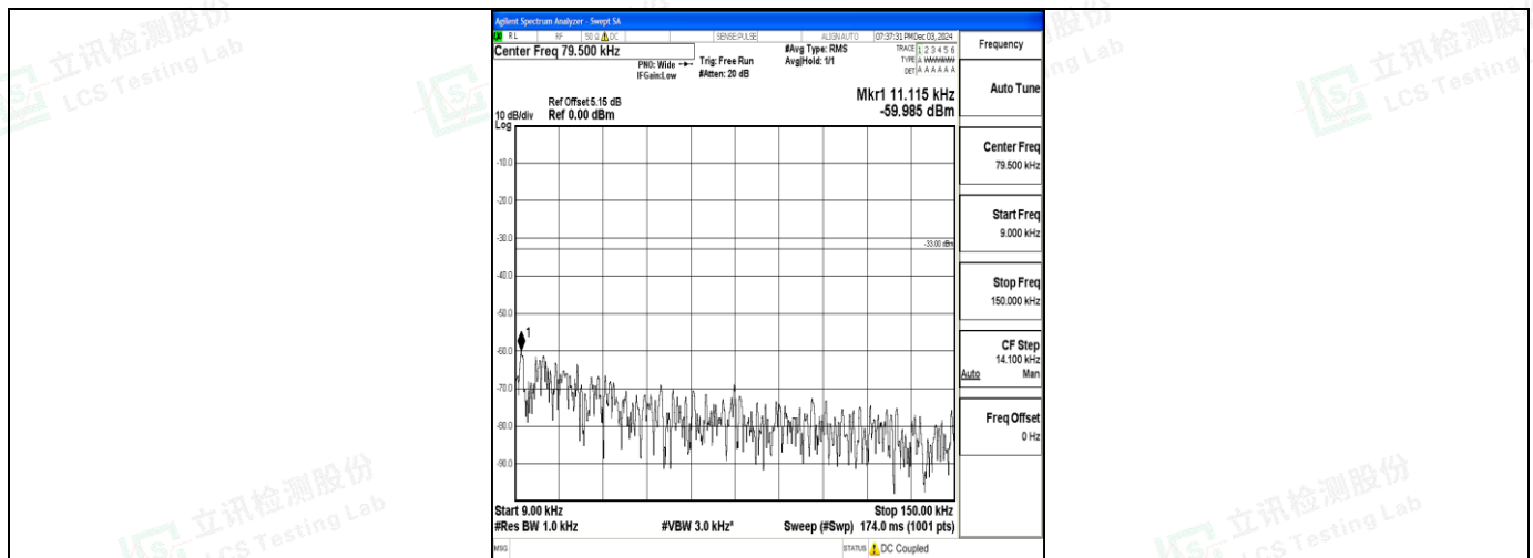
Band71_15MHz_QPSK_133397_1RB#0_0.009~0.15_0.009~0.15
