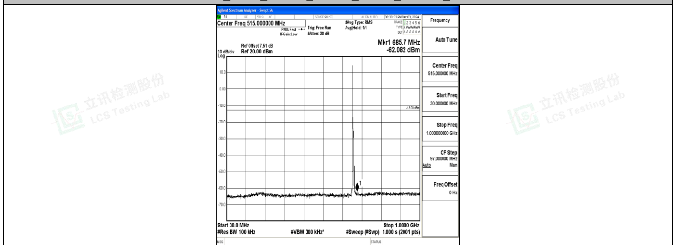
Band71_5MHz_16QAM_133147_1RB#0_30~1000_30~1000
