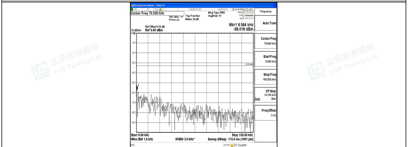
Band71_5MHz_QPSK_133297_1RB#0_0.009~0.15_0.009~0.15
