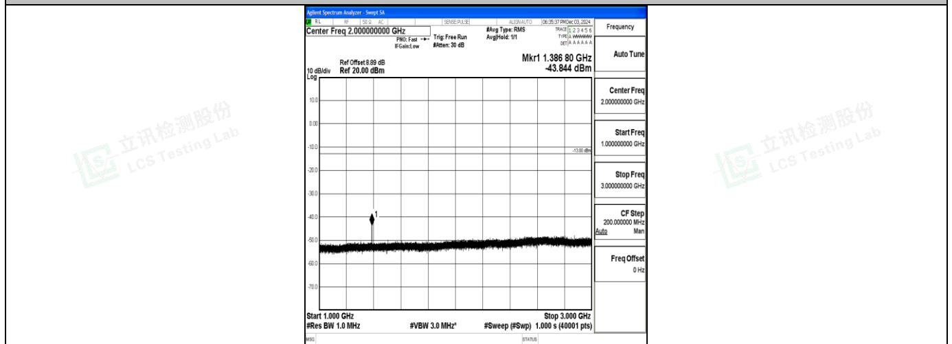
Band71_5MHz_16QAM_133447_1RB#0_1000~3000_1000~3000
