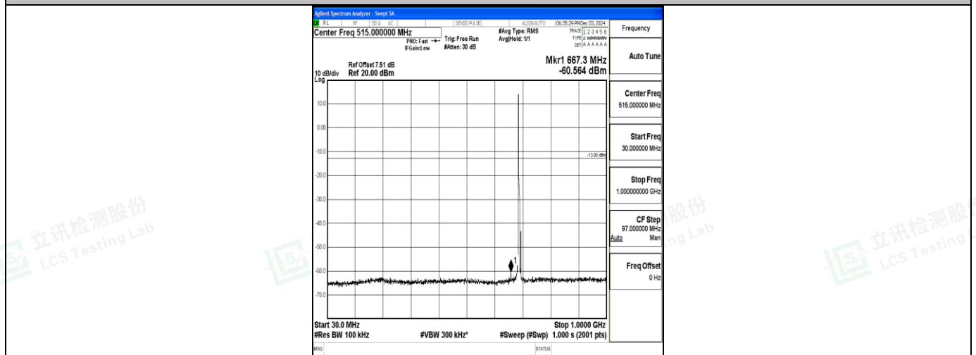
Band71_5MHz_16QAM_133447_1RB#0_30~1000_30~1000
