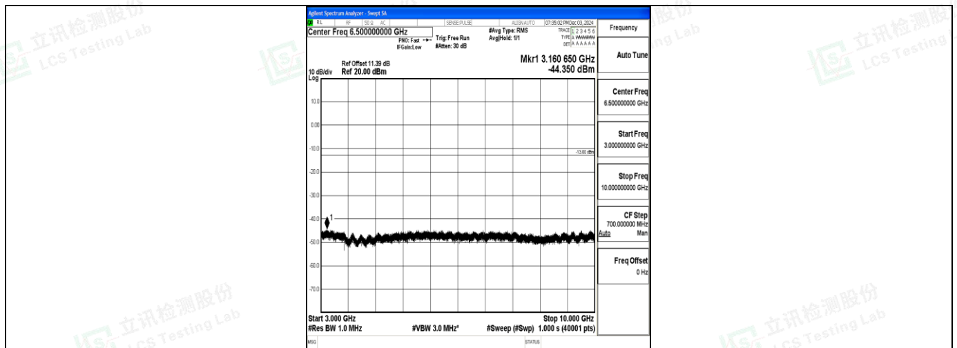
Band71_15MHz_QPSK_133297_1RB#0_3000~10000_3000~10000
