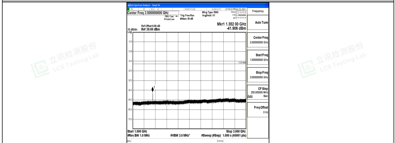
Band71_10MHz_QPSK_133297_1RB#0_1000~3000_1000~3000
