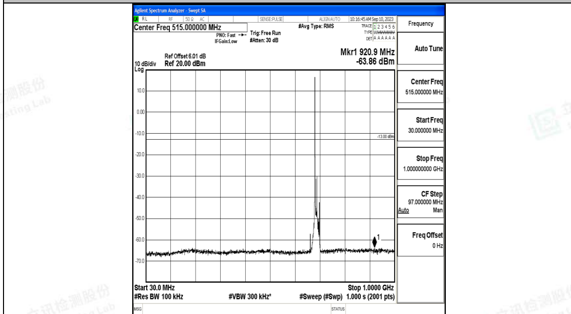
Band71_10MHz_16QAM_133422_1RB#0_30~1000_30~1000
