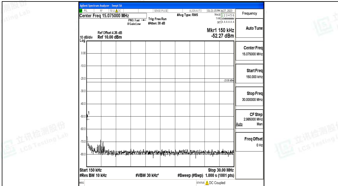
Band71_20MHz_16QAM_133222_1RB#0_0.15~30_0.15~30
