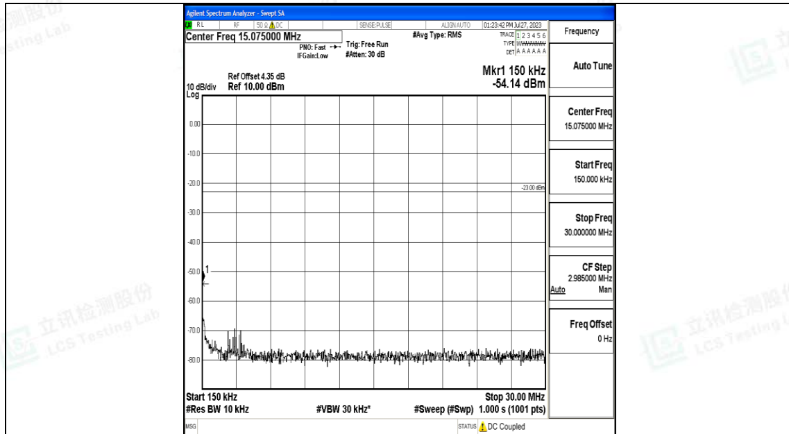
Band71_20MHz_16QAM_133372_1RB#0_0.15~30_0.15~30
