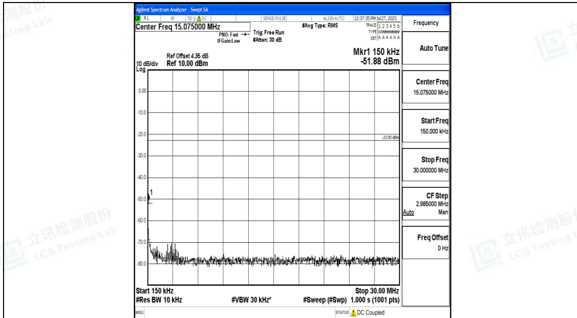
Band71_10MHz_16QAM_133297_1RB#0_0.15~30_0.15~30
