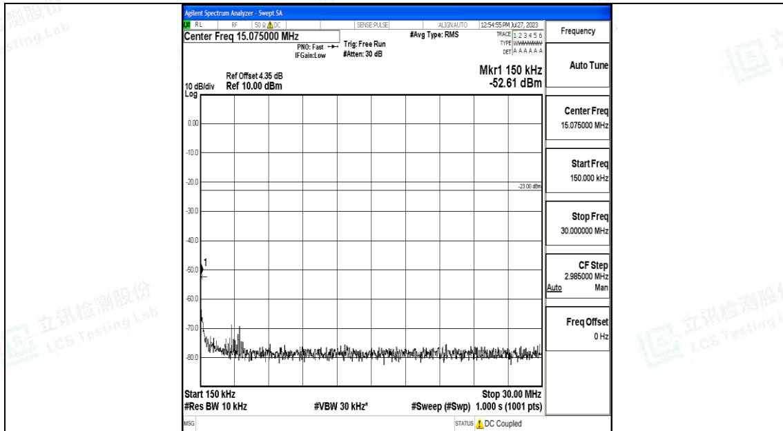
Band71_15MHz_16QAM_133397_1RB#0_0.15~30_0.15~30
