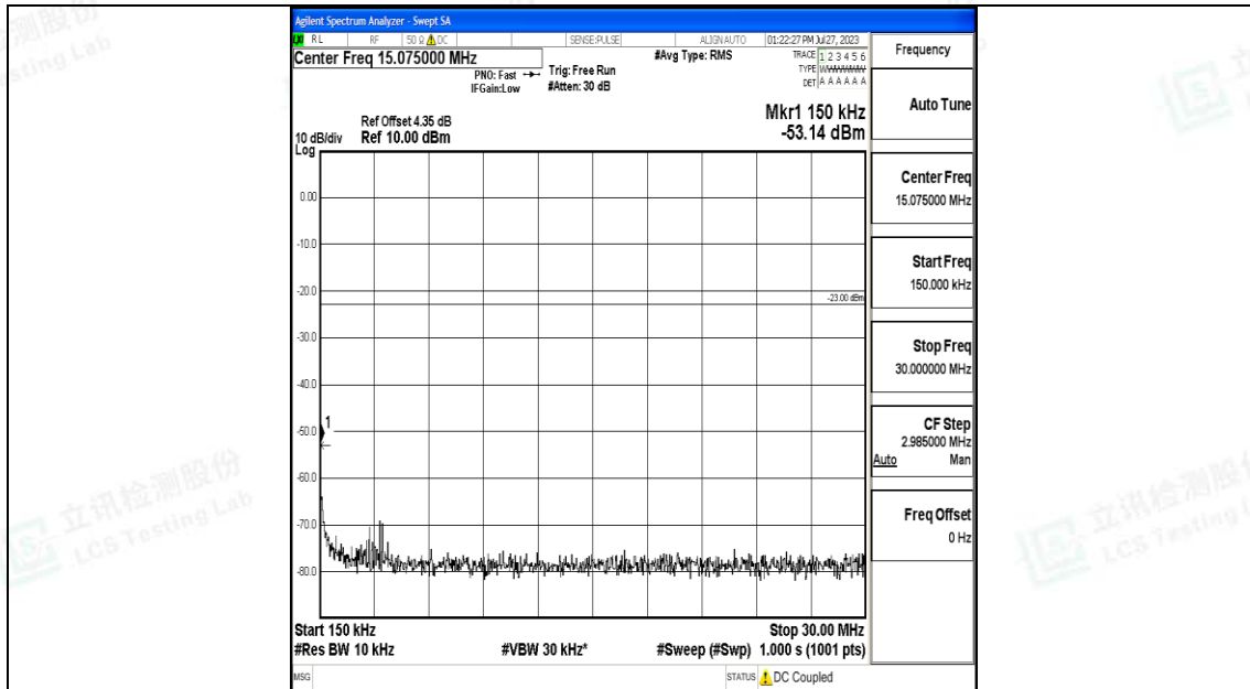
Band71_20MHz_16QAM_133322_1RB#0_0.15~30_0.15~30
