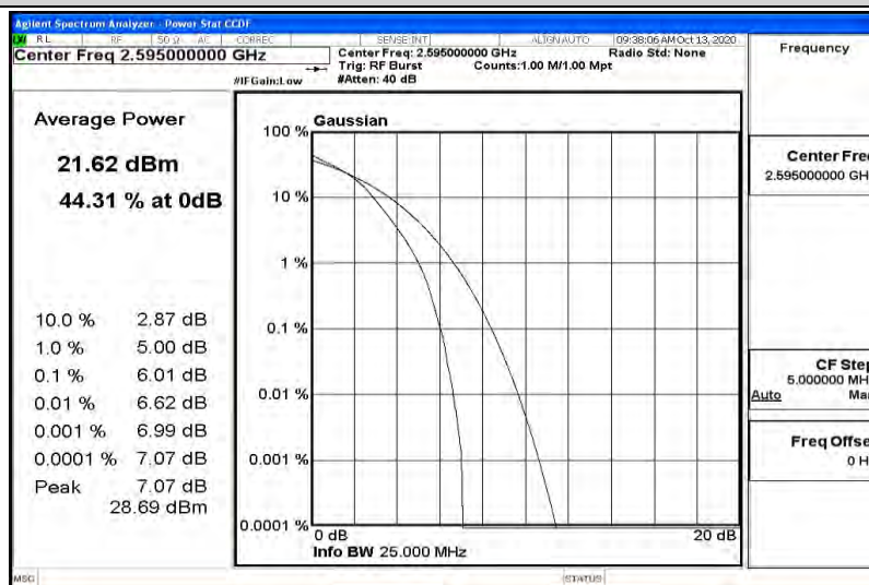
Band38-20MHz-16QAM-38150-1RB#0
