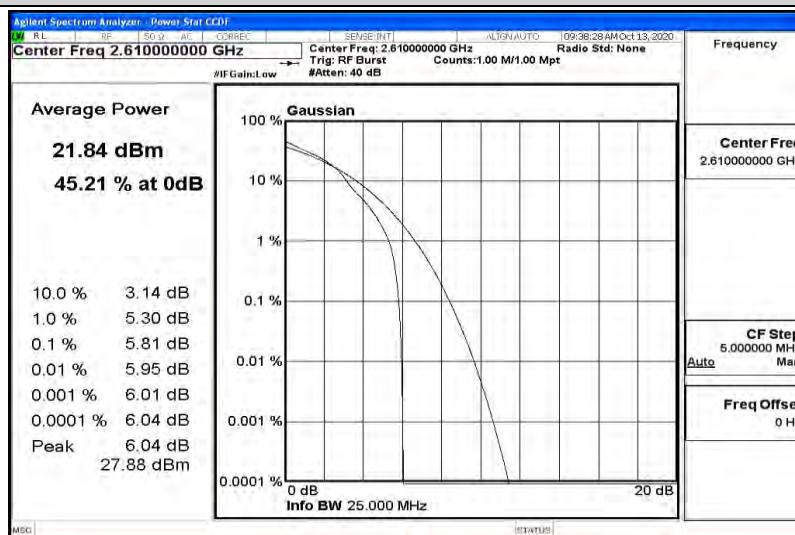
Band38-20MHz-16QAM-38150-100RB#0
