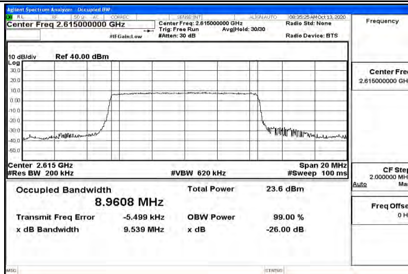
Band38-10MHz-16QAM-37800-50RB#0-8.9539
