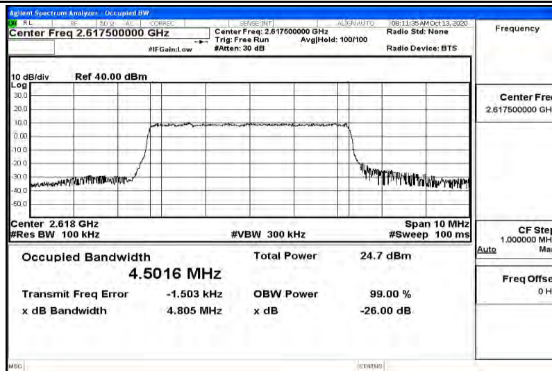
Band38-5MHz-16QAM-37775-25RB#0-4.4915
