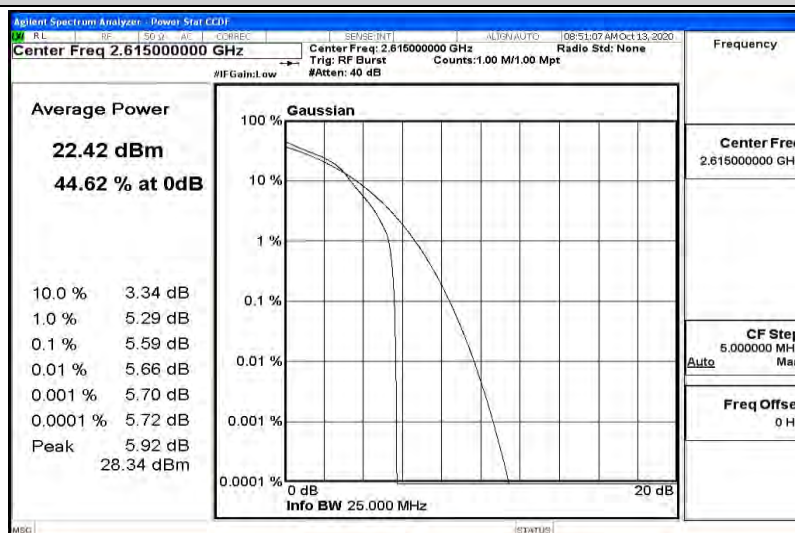
Band38-10MHz-16QAM-38200-50RB#0
