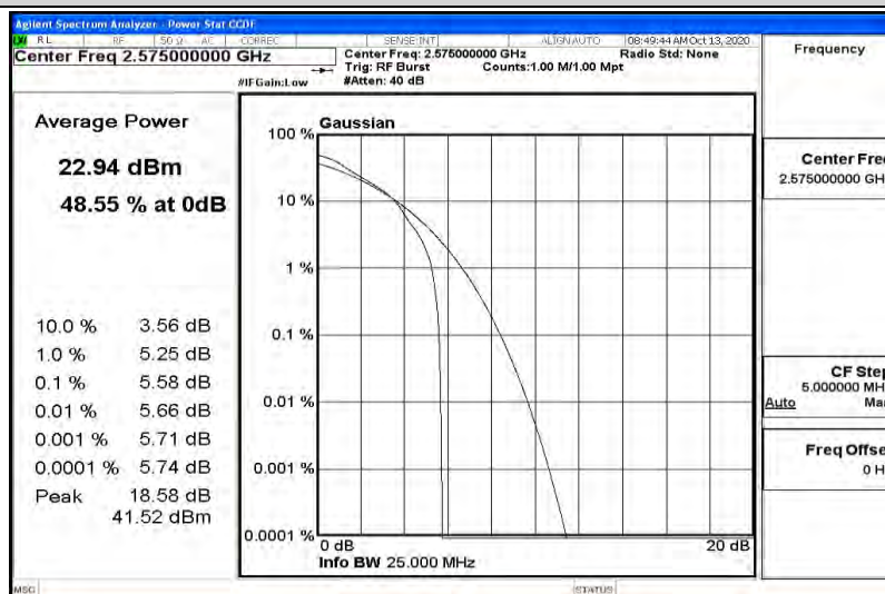
Band38-10MHz-QPSK-37800-50RB#0
