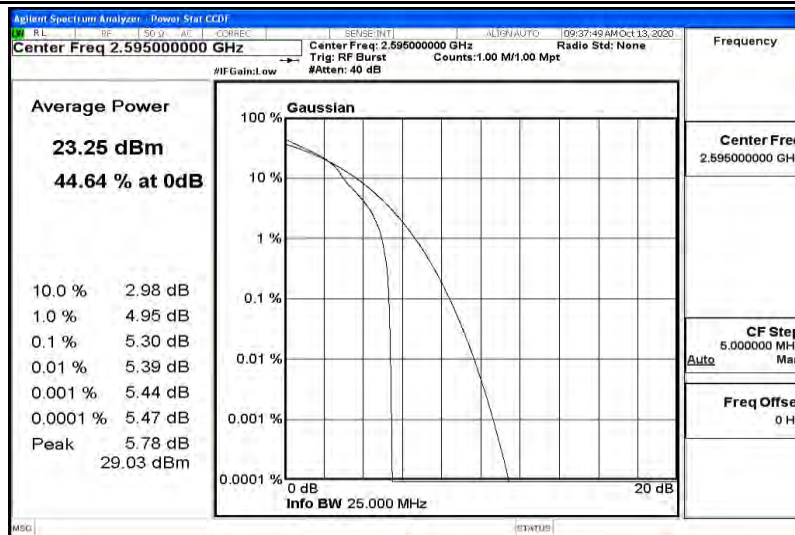
Band38-20MHz-16QAM-38000-100RB#0
