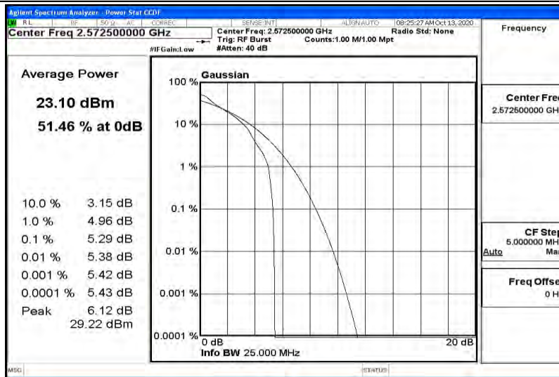
Band38-5MHz-QPSK-37775-25RB#0
