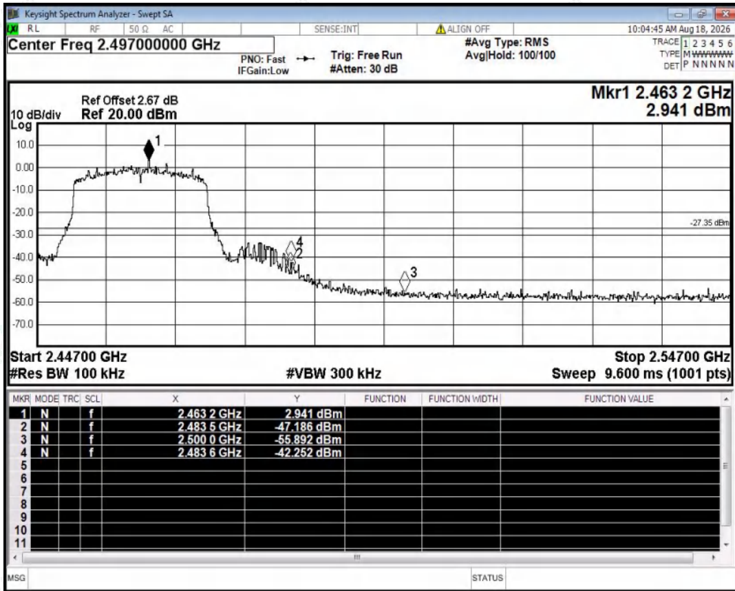
Band Edge NVNT ax20 2462MHz Ant1 Emission
