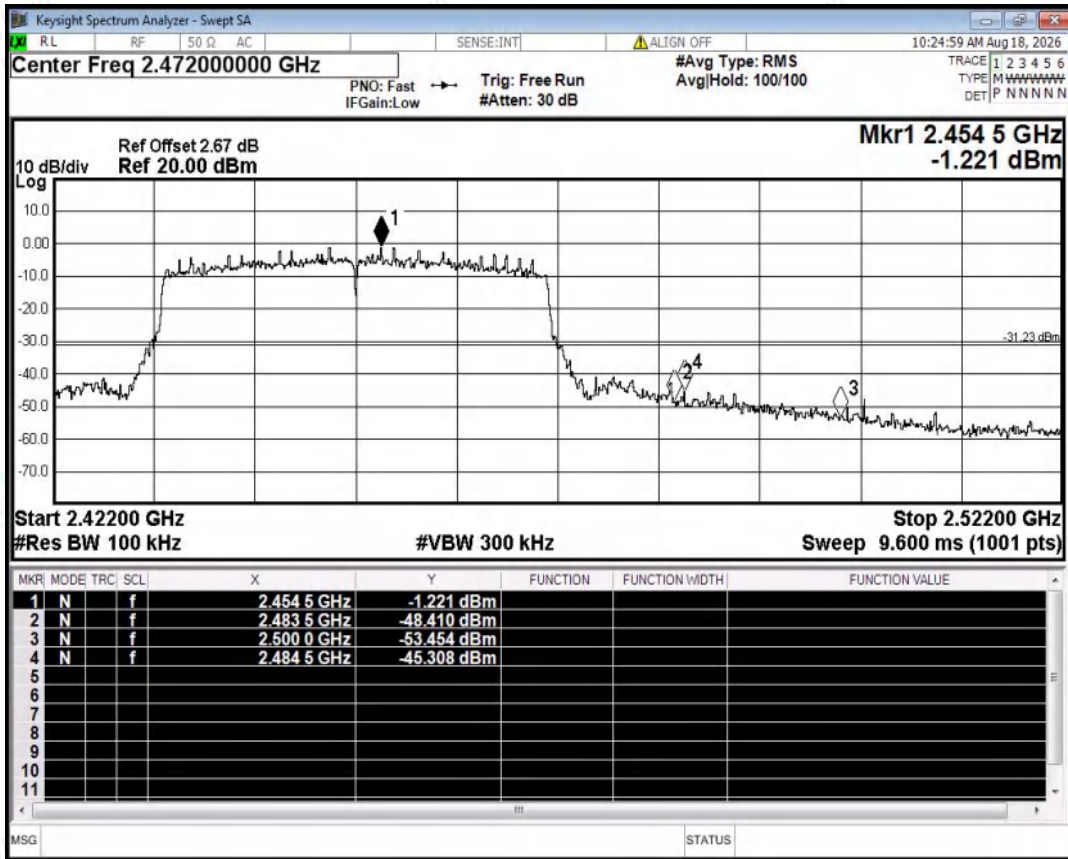
Band Edge NVNT ax40 2452MHz Ant1 Emission
