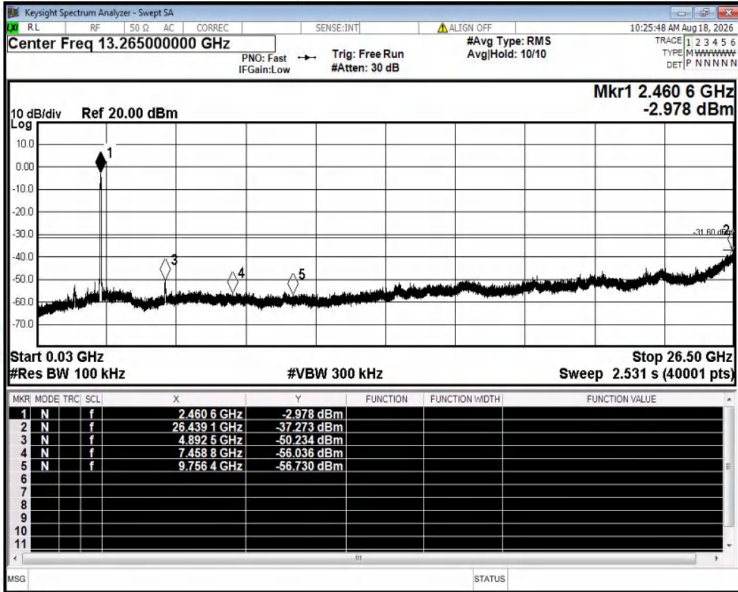
Tx. Spurious NVNT ax40 2452MHz Ant1 Emission
