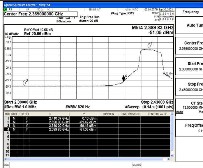
11G_Ant_Low_2412_Peak
