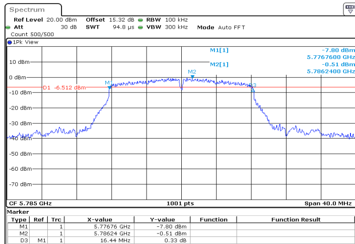
11A_Ant1_5785
