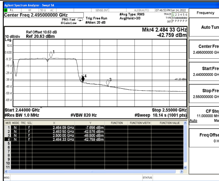
11N20SISO_Ant_High_2462_Peak
