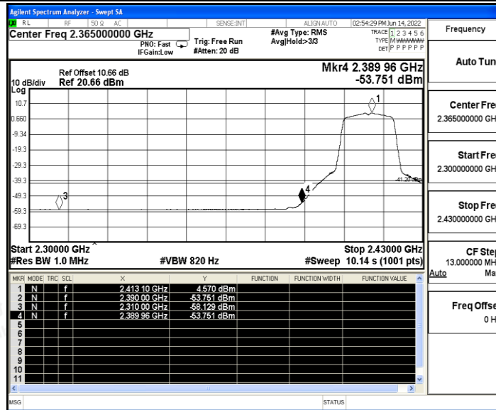
11G_Ant_Low_2412_Peak
