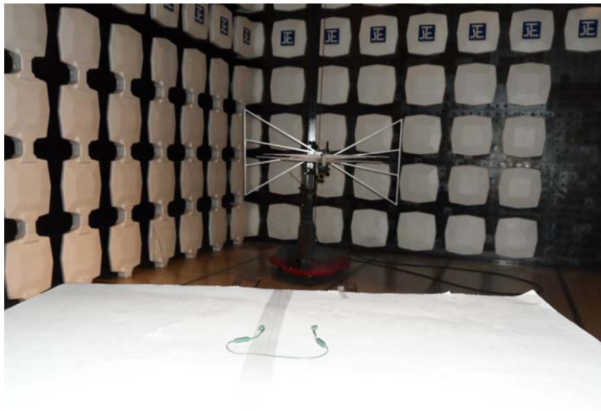
Measurement of Radiated Emission Test Set Up
