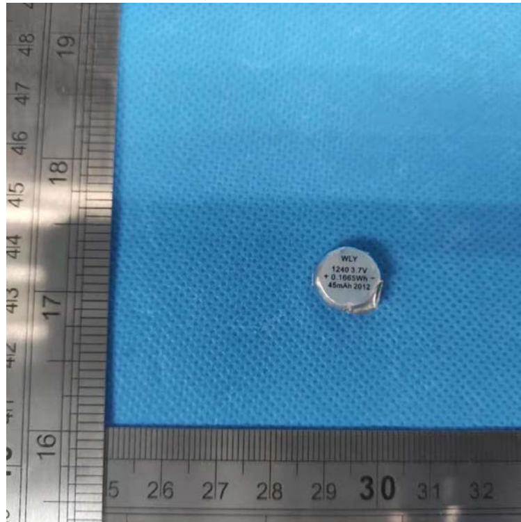
Battery View of the Product
