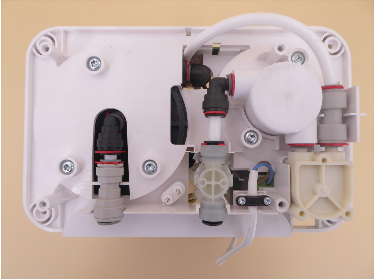
EUT, bottom view, bottom cover removed
