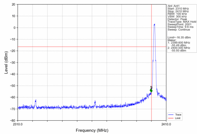
1M_LCH_2402MHz_Ant1_NTNV
