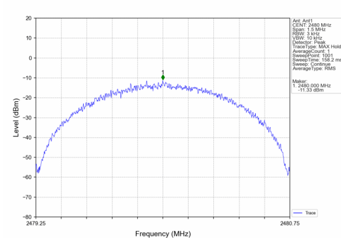
1M_HCH_2480MHz_Ant1_NTNV
