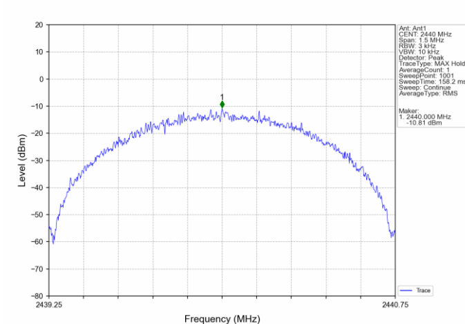
1M_MCH_2440MHz_Ant1_NTNV
