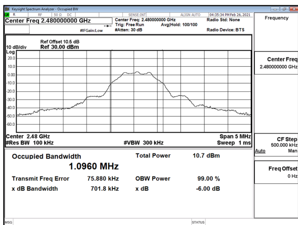
OBW 6dB_BLE_1M_HighCH39-2480
