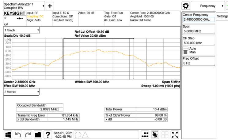
OBW 6dB_BLE_2M_HighCH39-2480
