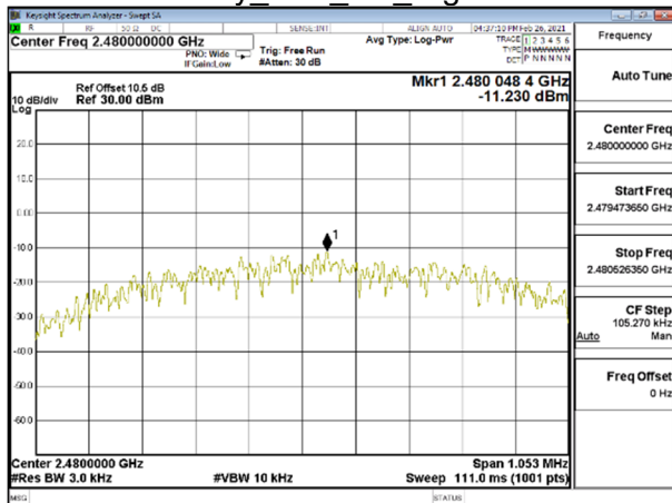
Power Density_BLE_1M_HighCH39-2480
