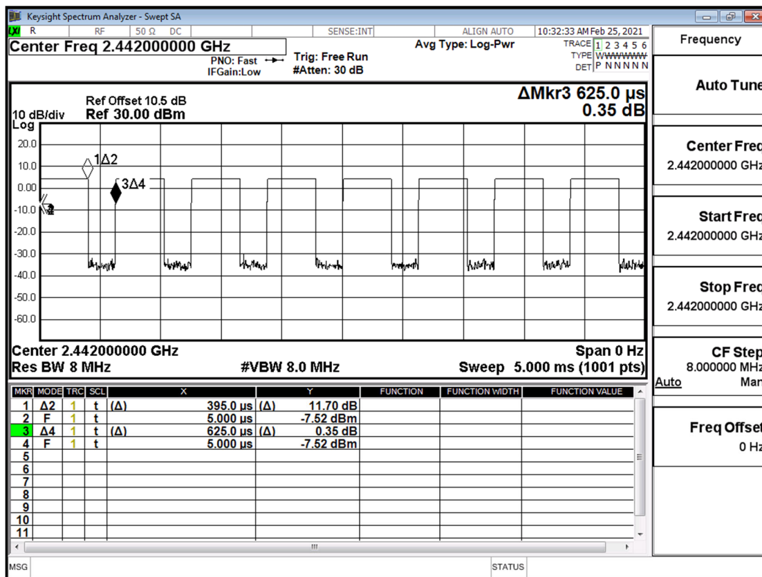
Duty Cycle_BLE_1M_MidCH20-2442
